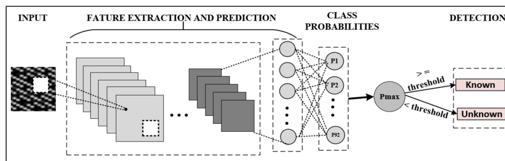
Figure 4. Framework to detect unknown in-app activity data.
