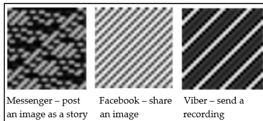
Figure 1. Grayscale images generated from the encrypted in-app activity data.
