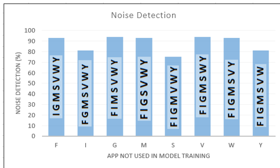
Figure 5. Noise detection rates of unknown apps.
