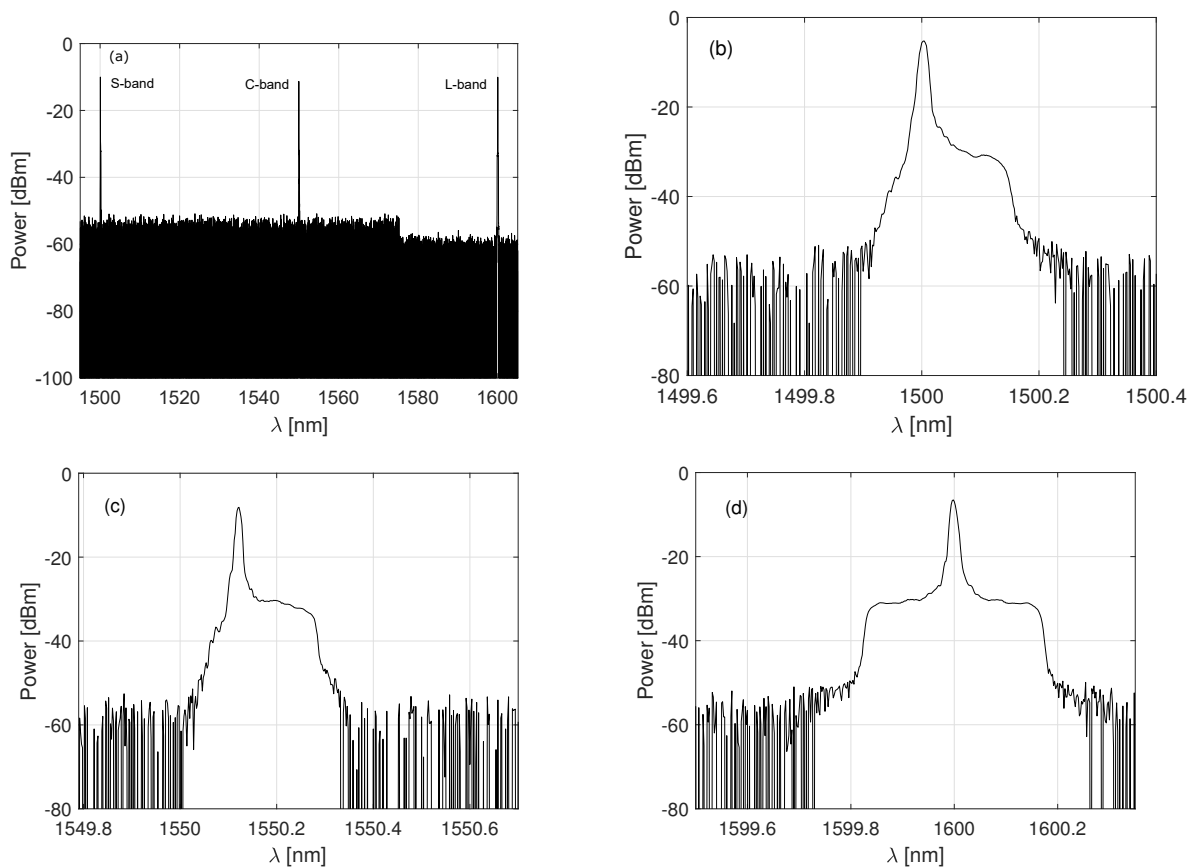
Figure 6. (a) Transmitted MB high-capacity flow after MB(oSDM) S-BVT optical aggregator; (b) S-band SSB; (c) C-band SSB; (d) L-band DSB-transmitted spectra.
