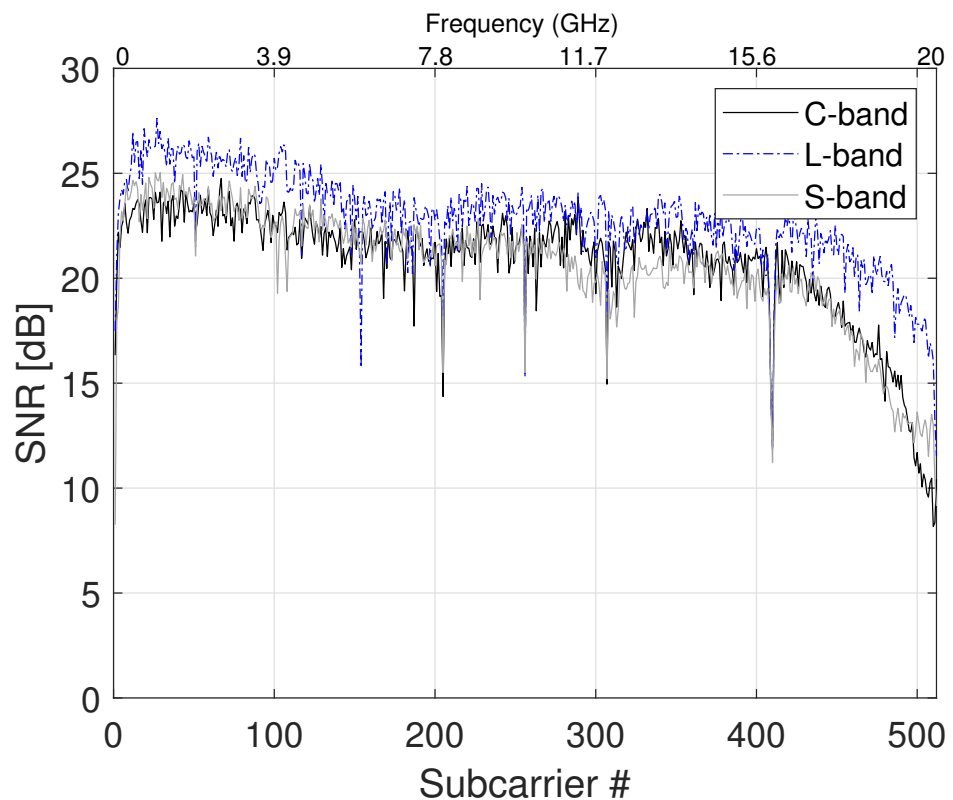
Figure 7. SNR profile of the S-, C-, and L-band contributions in B2B configuration.
