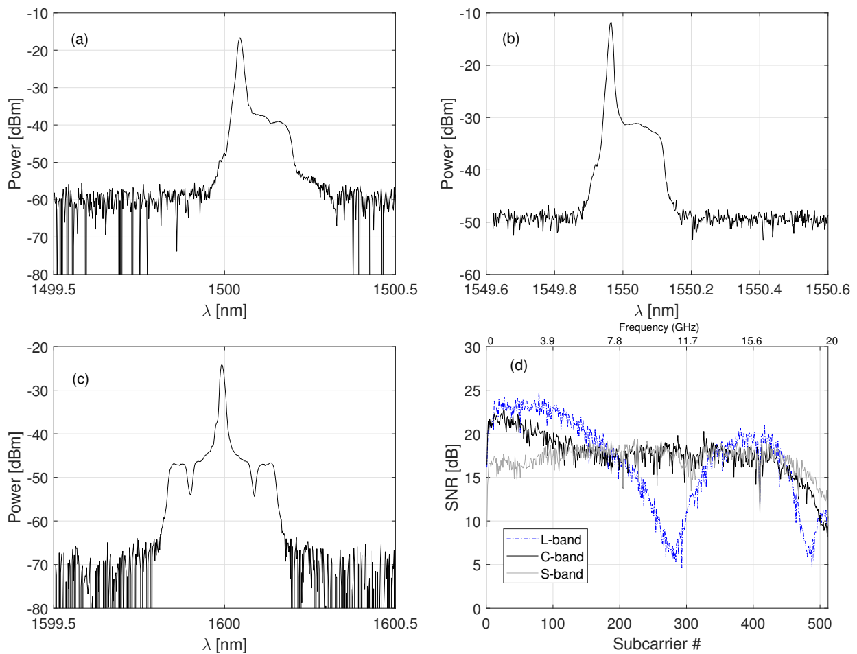
Figure 8. OSA captures after applying BPL and after 25 km of SSMF of the (a) S-band (b) C-band, and (c) L-band slices. (d) SNR profile of the S-, C-, and L-band contributions after 25 km of SSMF.
