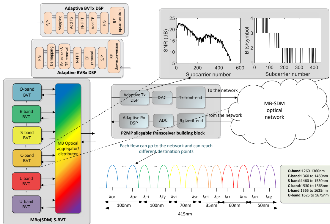
Figure 1. MB(oSDM) S–BVT architecture.
