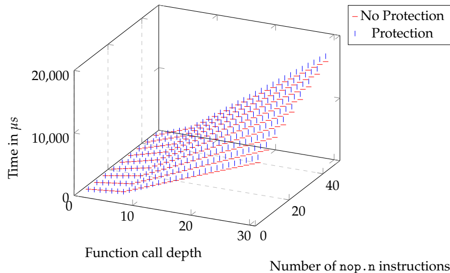
Figure 9. Synthetic benchmark runtimes in \mu s based on the call depth and the number of nop.n instructions in the function with and without the window-overflow protection
