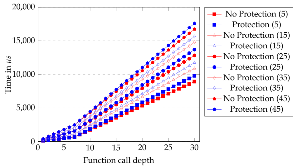
Figure 8. Selected synthetic benchmark runtimes in \mu s based on the call depth and the number of nop.n instructions in the function (noted in parenthesis) with and without the window-overflow protection.
