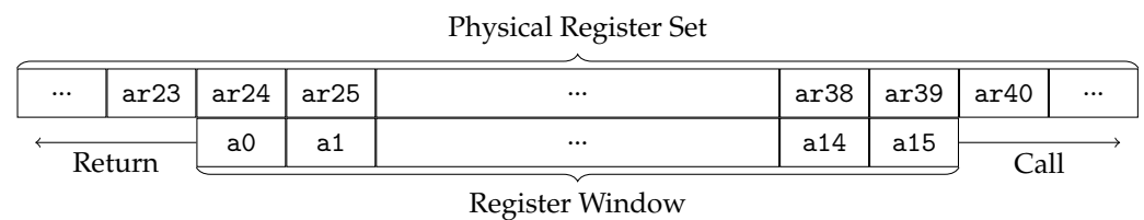
Figure 1. Example of a register window mapping of logical registers a0–a15 to physical registers ar24–ar39.
