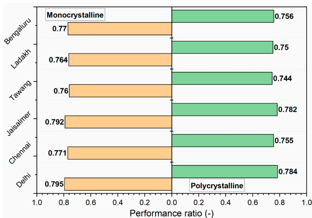
Figure 11. Performance ratio for the station in all six cities with different module technologies.
