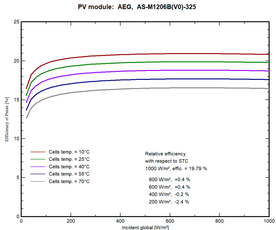
Figure 5. Efficiency curve for the selected monocrystalline module.
