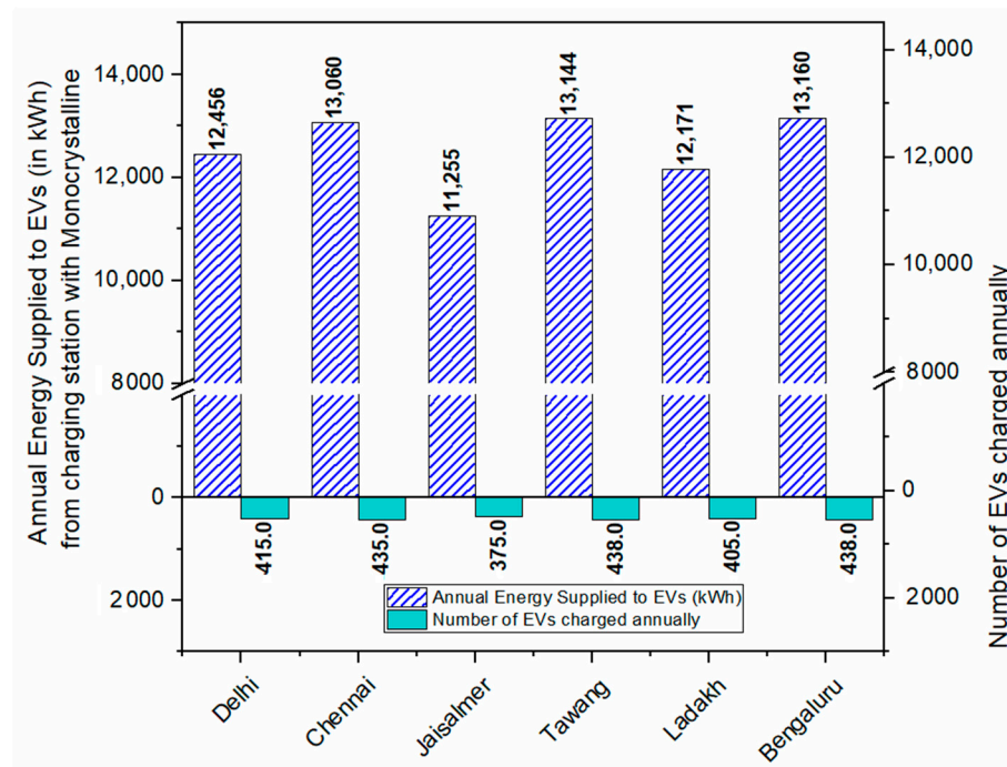
Figure 14. Annual energy supplied to EVs by the charging station using monocrystalline panels.
