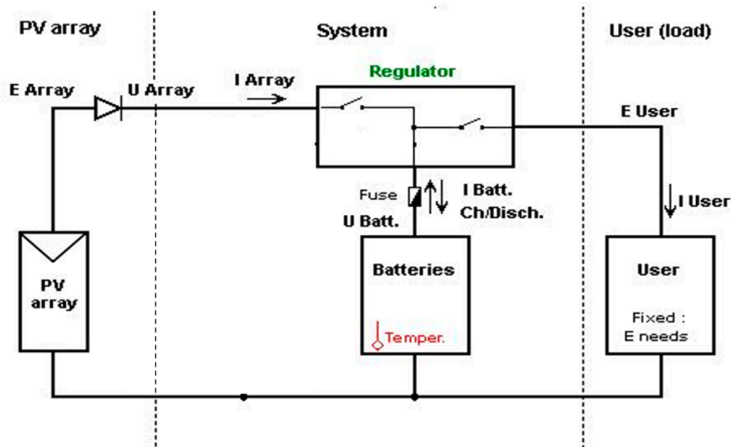
Figure 10. Single line diagram of the charging station.
