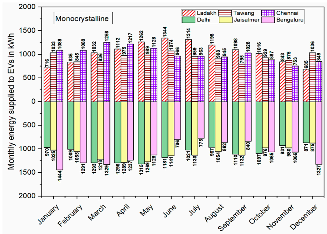
Figure 12. Monthly variation in energy supplied to EVs by the charging station using monocrystalline modules.
