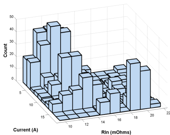
Figure 9: Cell #11 R_{in} count versus Current
