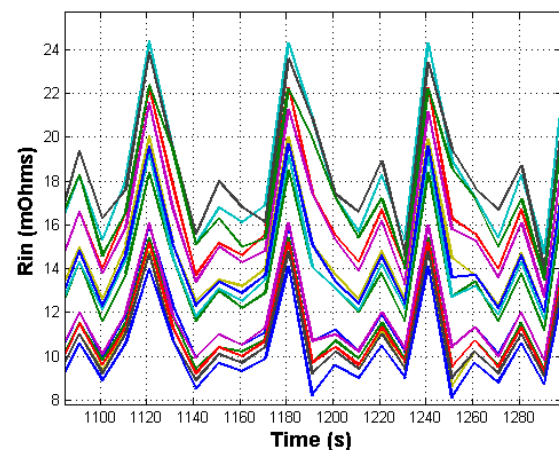
Figure 7: R_{in} Measurement
