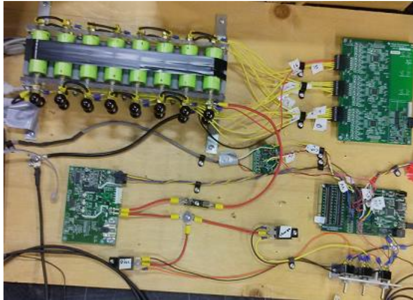
Figure 4: The bench test
