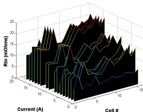
Figure 8: R_{in} versus Current comparison
