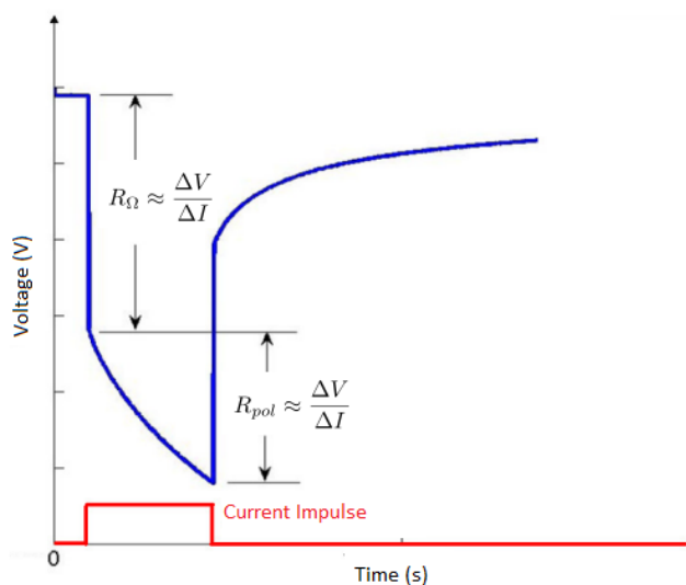
Figure 2: Estimation of R_{in} , R_{\Omega} and R_{pol} [11]
