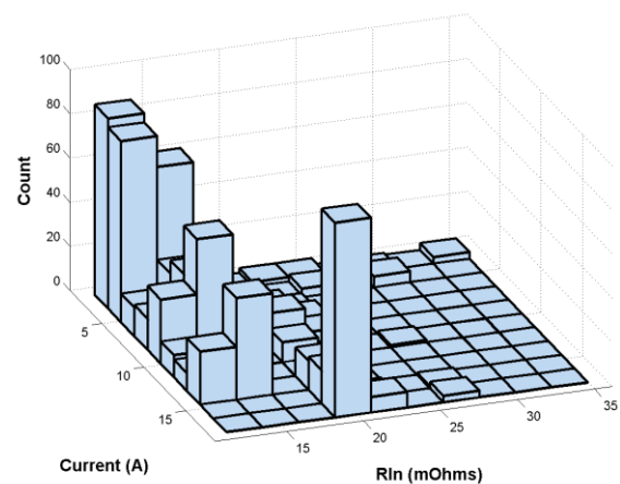
Figure 10: Cell #13 R_{in} count versus Current
