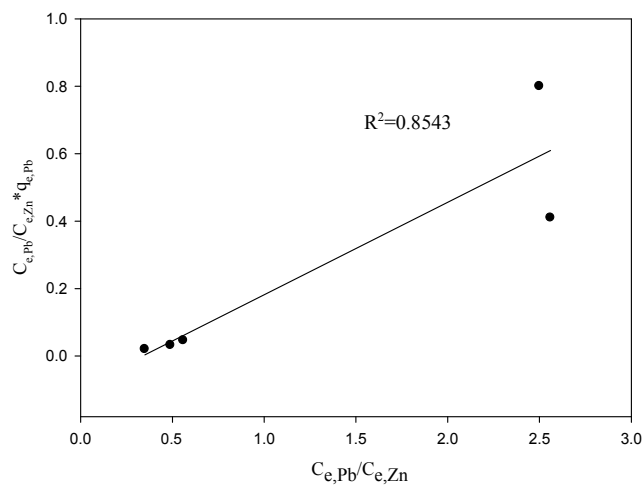
(b) Sorption of Pb^{2+} in the presence of Zn^{2+}
