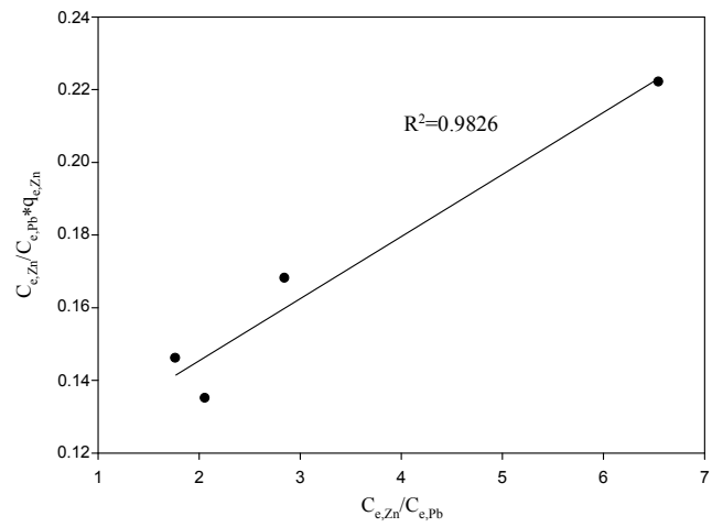
(a) Sorption of Zn^{2+} in the presence of Pb^{2+}
