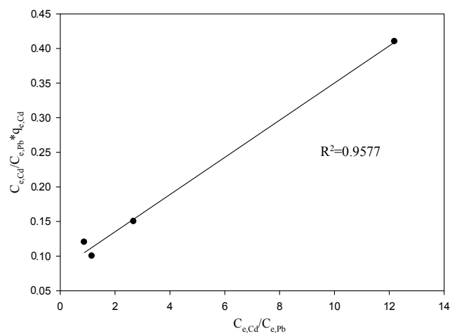
(c) Sorption of Cd^{2+} in the presence of Pb^{2+}
