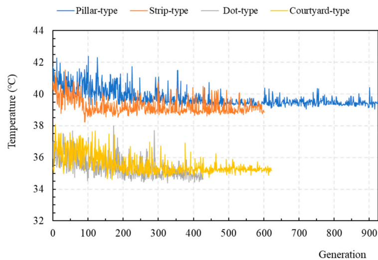
Figure 12. Variation trend of the MRT of the four block types.
