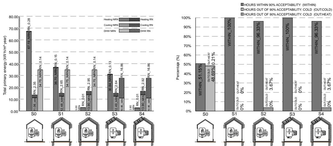
Figure 9. Primary energy use (left) and percentage of hours within the 90% of acceptability comfort range (right) in Alferez Rojas case study (S#: scenario #; NRN: nonrenewable; RN: renewable).
