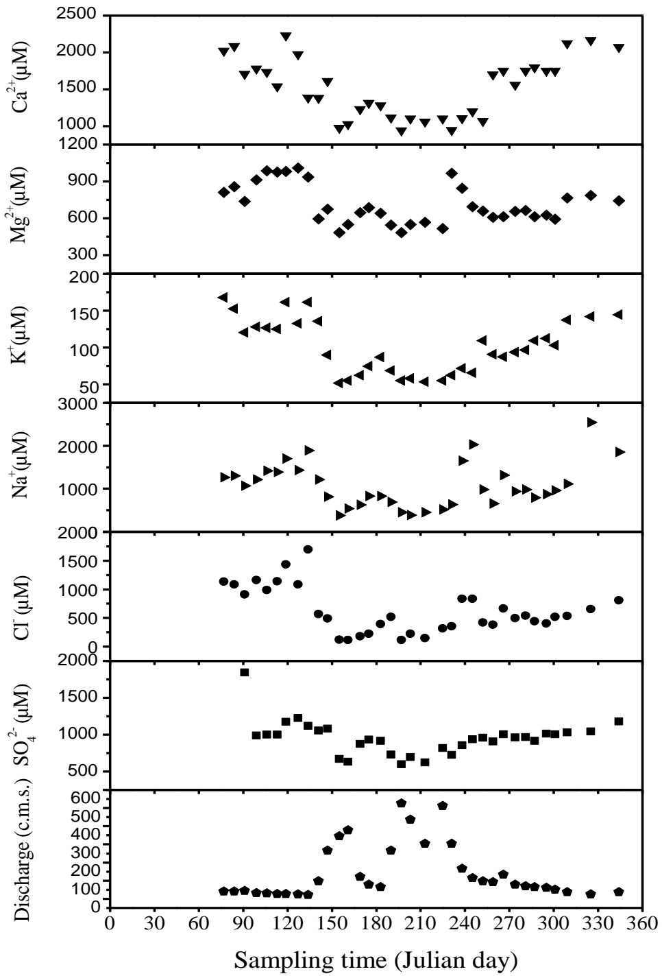
Figure S1. Temporal variability of dissolved major ions and discharge in the river end-member (Station 11) in 2002.
