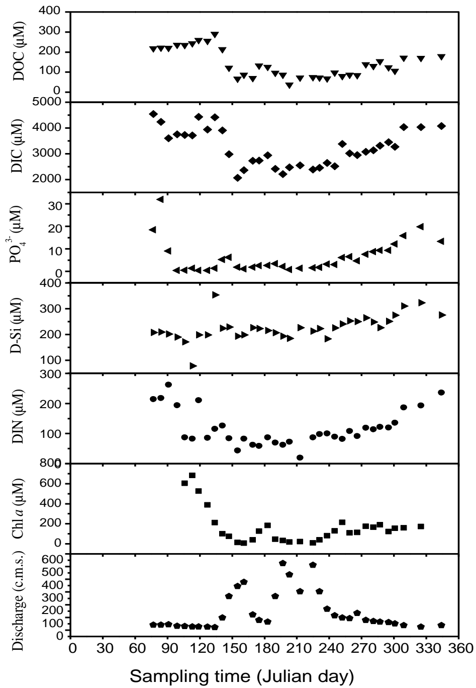
Figure S2. Temporal variability of DIC, DOC, nutrients, Chl-a and discharge in the river end-member (Station 11) in 2002.
