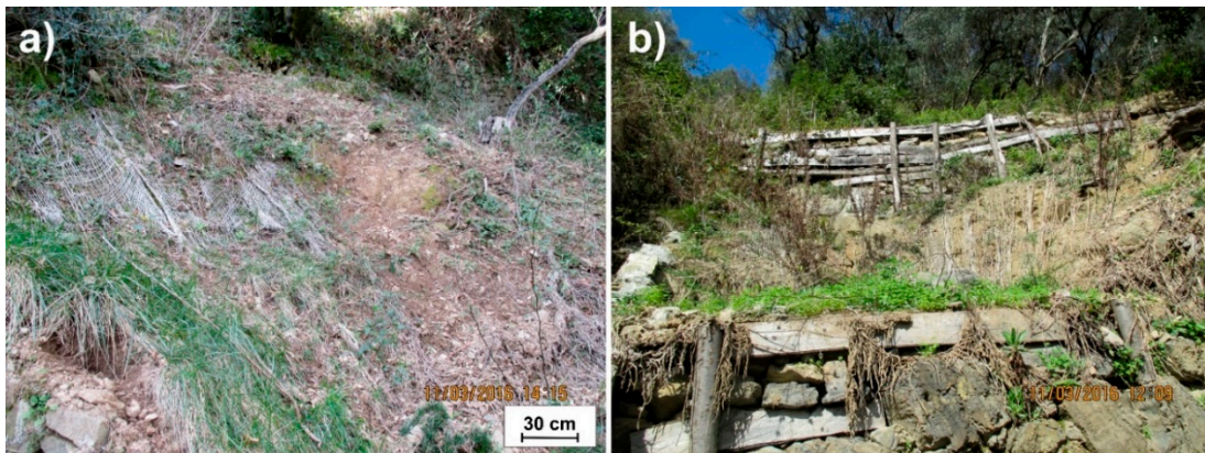
Figure 12. Examples of scarce vegetation cover development along a slope surface (a) and within single palisades (b).
