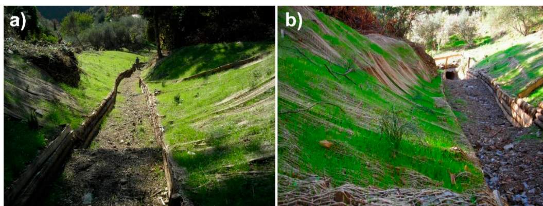
Figure 9. (a) Example of channel flanks stabilized with the combination of jute netting, grass sowing and shrub planting. (b) Detailed view of planted broom species on a stream bank (photos courtesy of Monterosso al Mare Municipality Administration).
