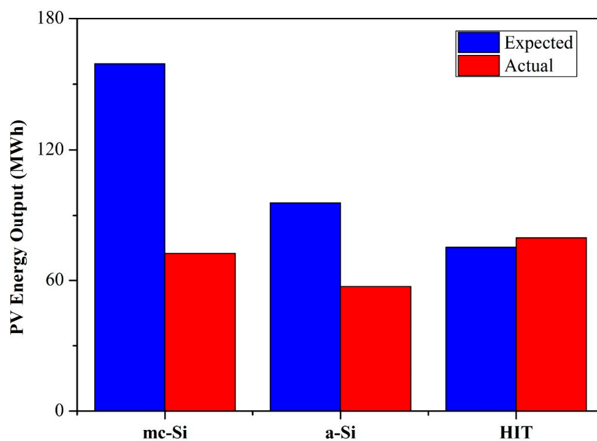
Figure 8. Actual VS Expected PV energy generation.
