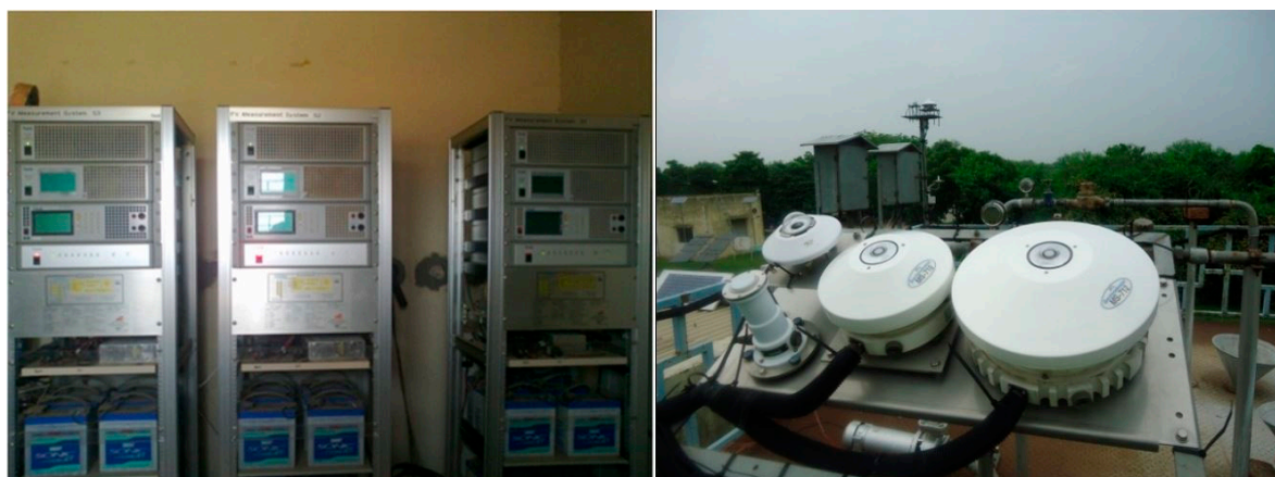
Figure 3. PV measurement system and meteorological data recording facilities.
