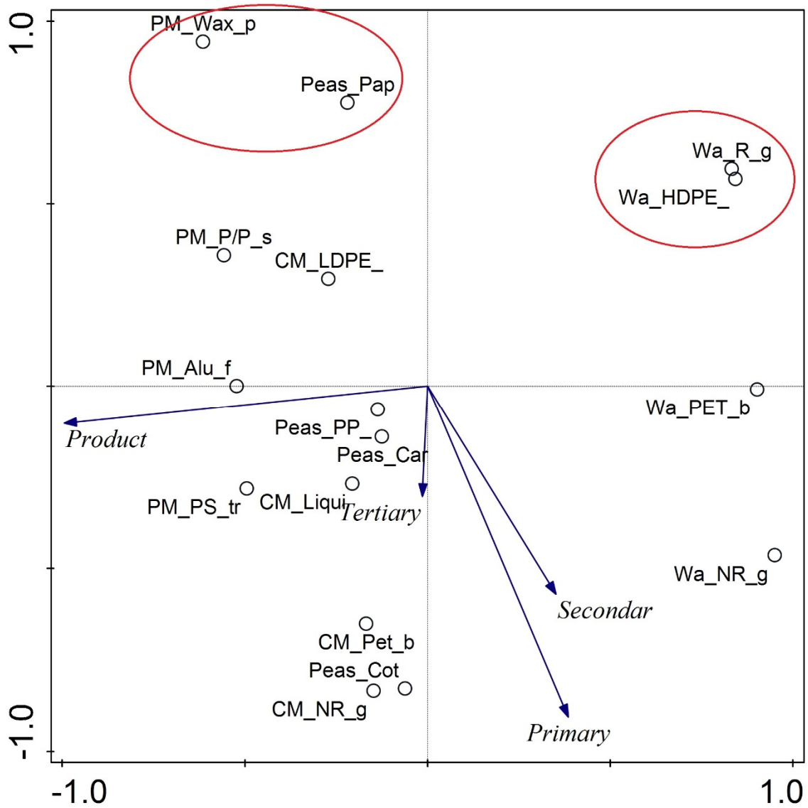
Figure S1. Principal component analysis of variations of climate change impact for different types of packaging and products for Energy Recovery Scenario.
