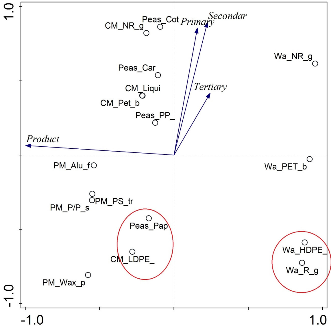
Figure S3. Principal component analysis of variations of climate change impact for different types of packaging and products for Landfilling Scenario.
