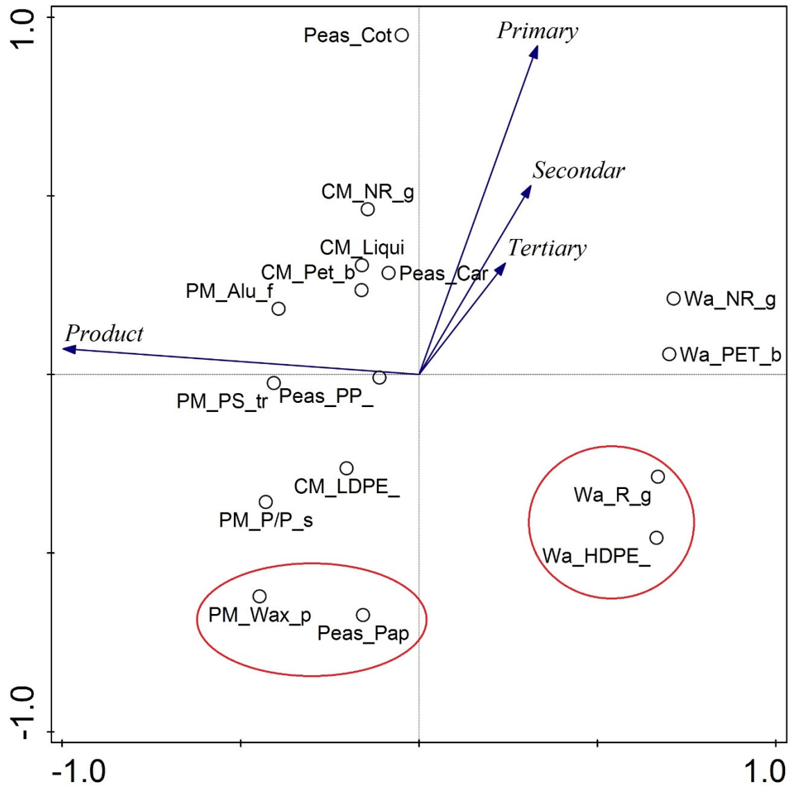
Figure S2. Principal component analysis of variations of climate change impact for different types of packaging and products for Material Recovery Scenario.
