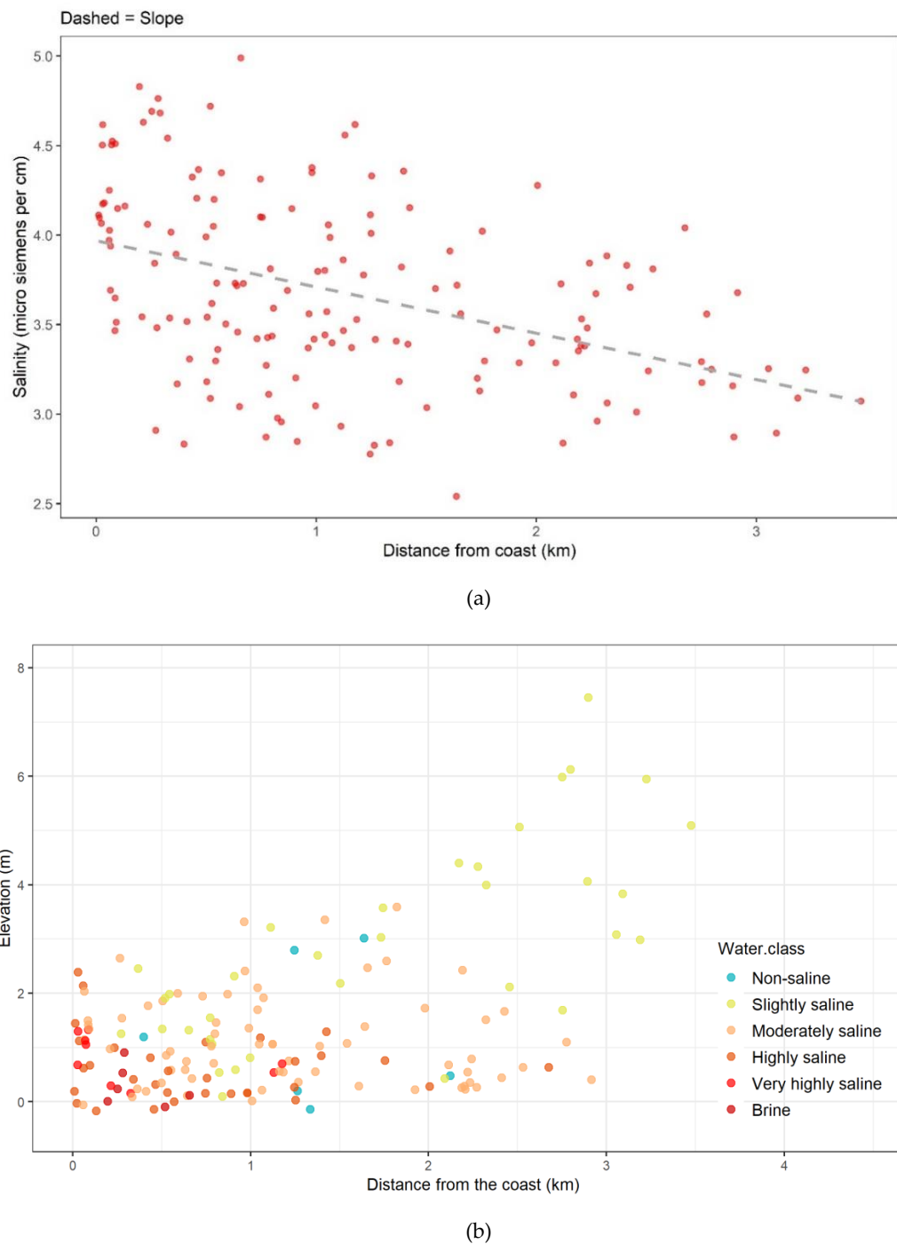
Figure 6. (a) Linear regression graph of salinity trend between EC of wells and their distance from the coast. (b) The scatterplot depicting elevation and distance of the 156 wells that were studied in 2019. The EC values ( \mu\text{S cm}^{-1} ) for the various wells is shown in different colour variations.
