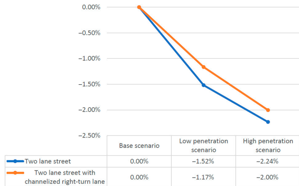
Figure 5. Changes in total delay per vehicle (%).
