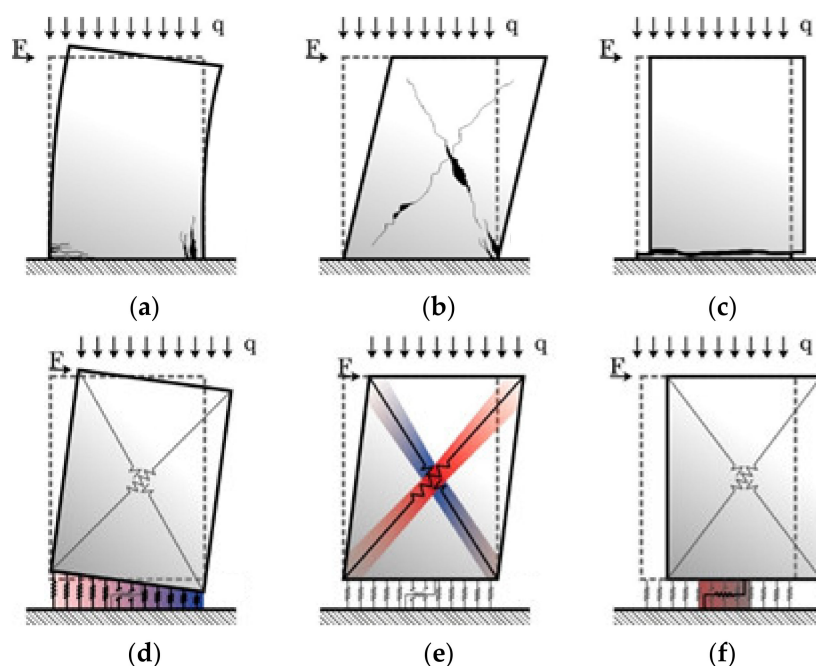
Figure 1. Main in-plane collapse mechanisms of masonry walls (top) and their simulation by means of the macro-element (bottom): (a–d) flexural failure; (b–e) shear-diagonal failure; and (c–f) shear sliding failure [15].
