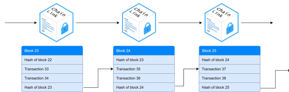
Figure 5. The structure of a blockchain.
