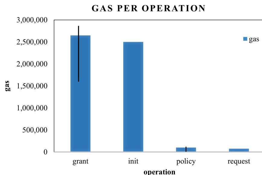
Figure 11. Gas per operation.
