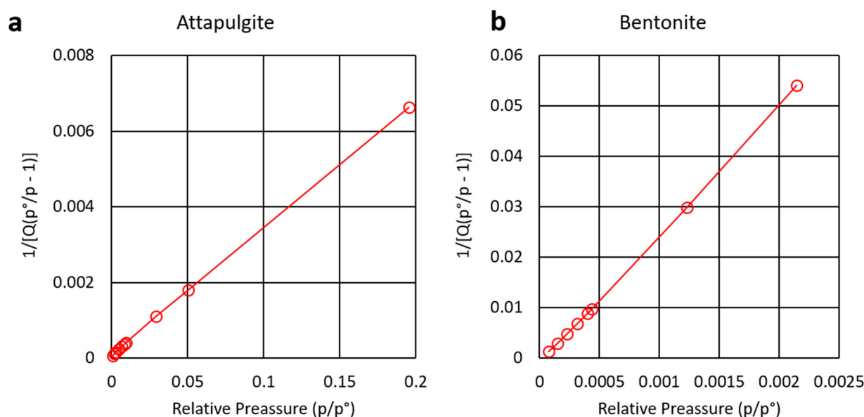
Figure 2. Brunauer-Emmett-Teller (BET) surface area plots for nitrogen gas adsorption on (a) attapulgite and (b) bentonite clay minerals.
