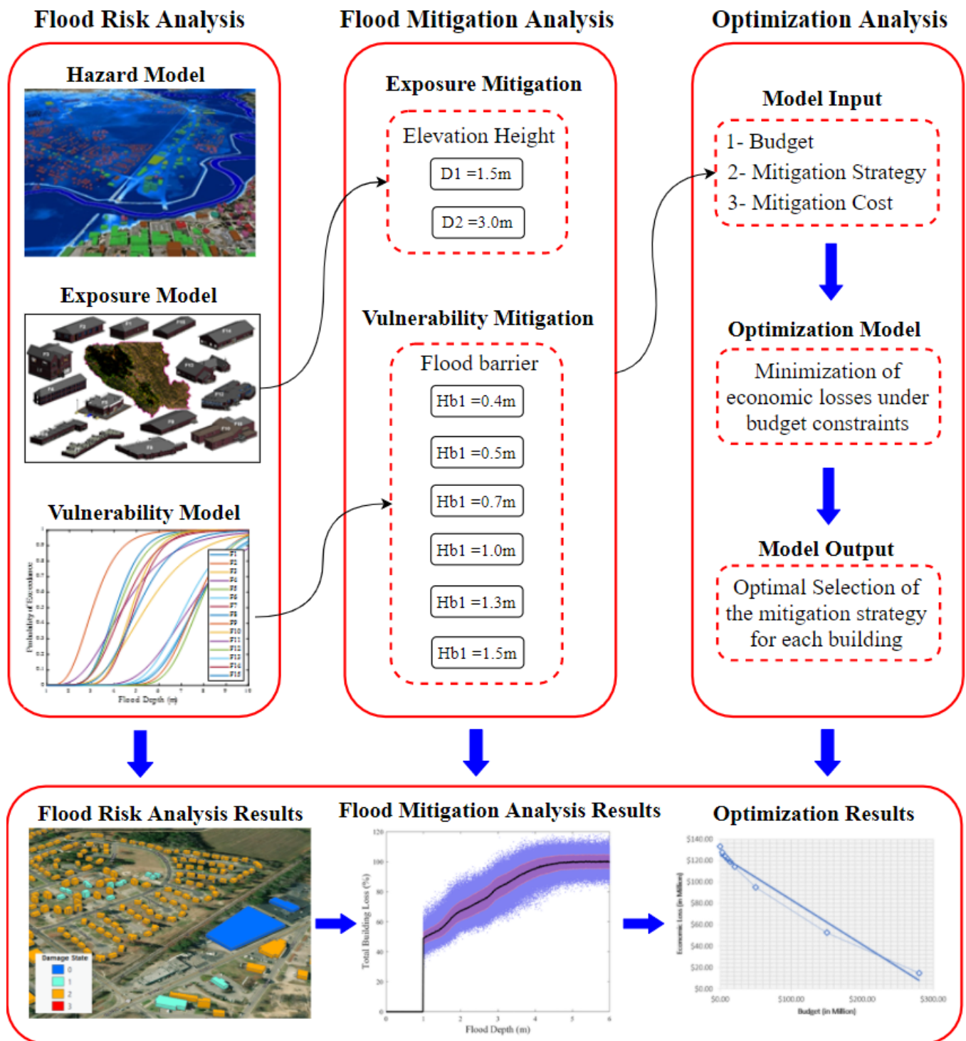
Figure 1. Schematic representation of the needed inputs for the optimization model.
