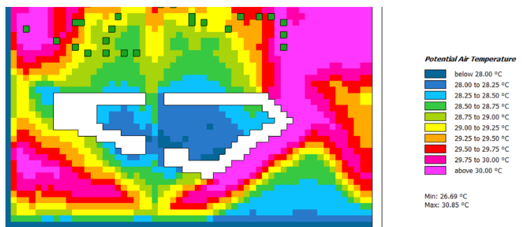
Figure 7. Envi-met simulation, Potential Air Temperature with emissivity equal to 0.5.
