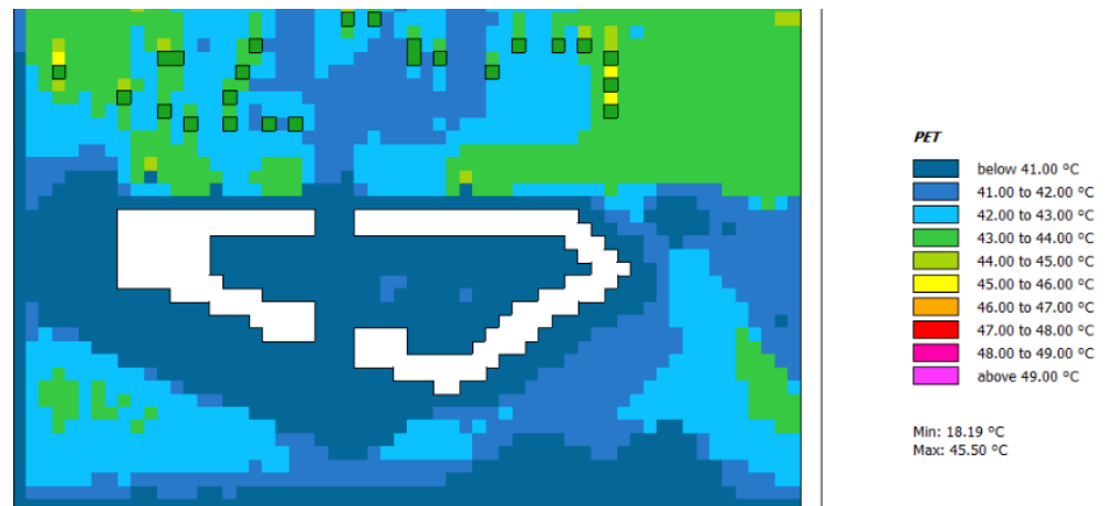
Figure 6. Envi-met simulation, PET with emissivity equal to 0.1.
