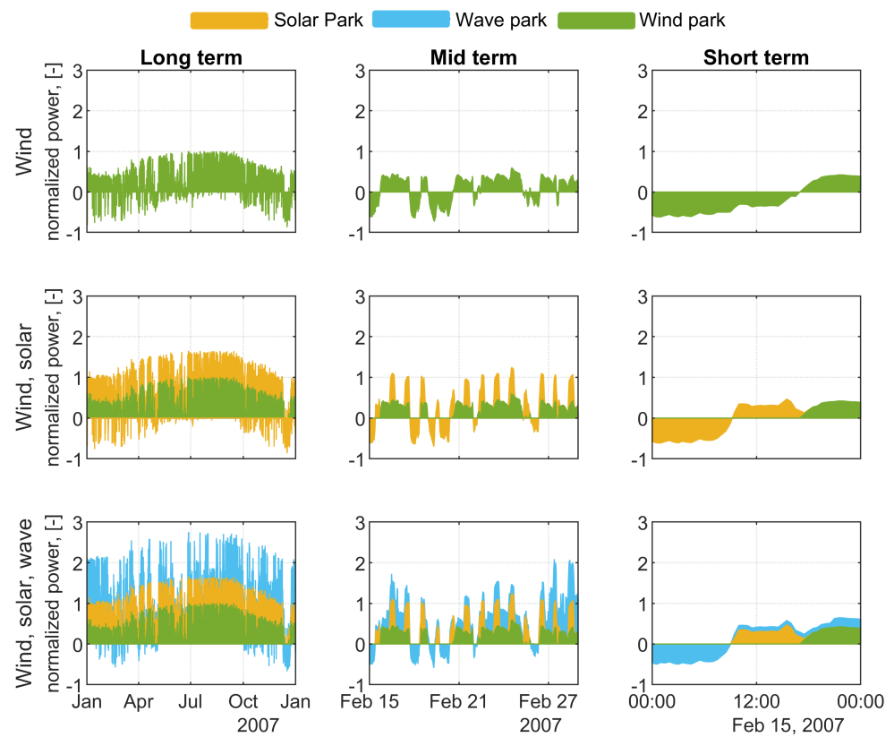
Figure 11. Net load in 2007: long, mid, and short (15 February) term. Wind power is denoted by green colour, two RESs (solar and wind) by yellow, and three RESs (wave, solar, and wind) by blue.
