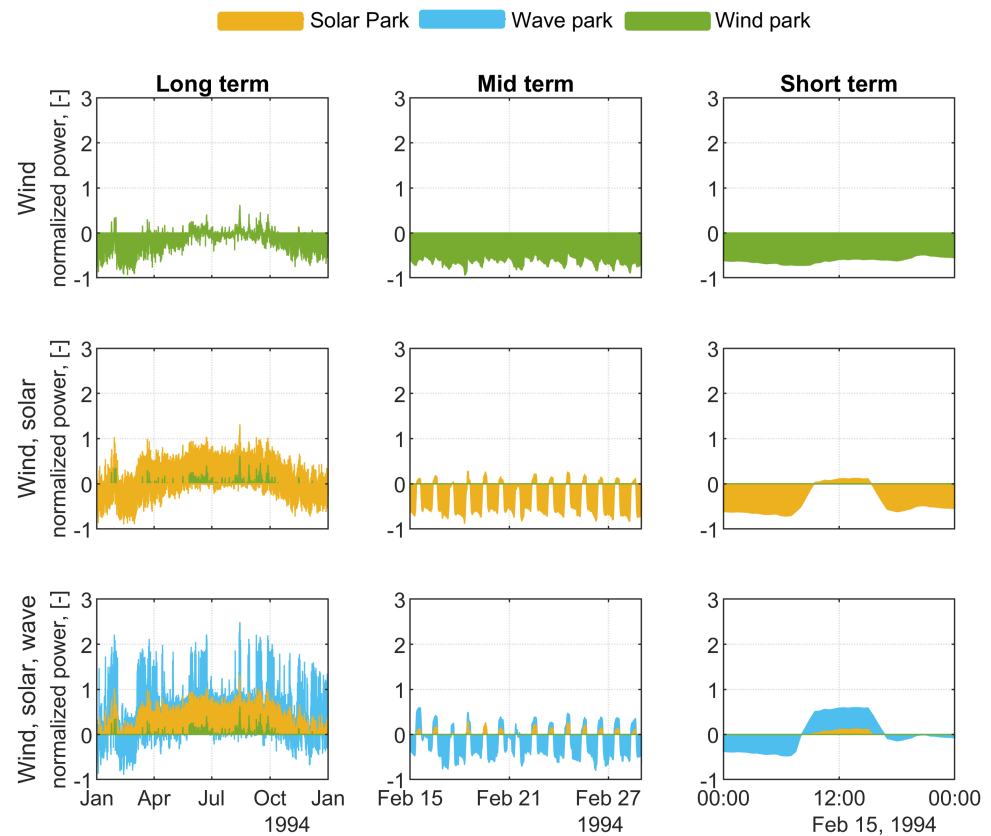
Figure 10. Net load in 1994: long, mid, and short (15 February) term. Wind power is denoted by green colour, two RESs (solar and wind) by yellow, and three RESs (wave, solar and wind) by blue.
