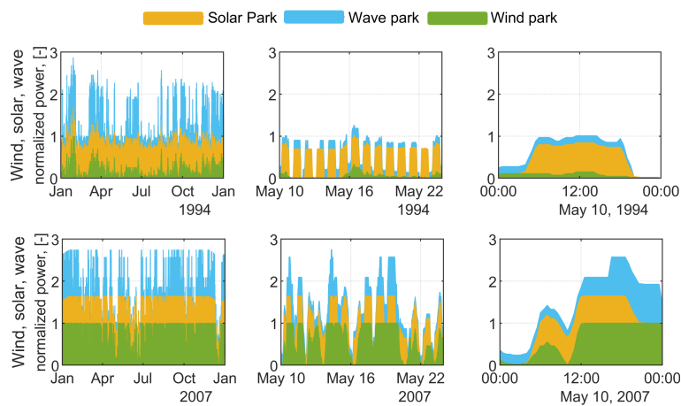
Figure 8. RESs supply in 1994 and 2007: long, mid, and short term (10 May). Wind power is denoted by green colour, two RESs (solar and wind) by yellow, and three RESs (wave, solar, and wind) by blue.
