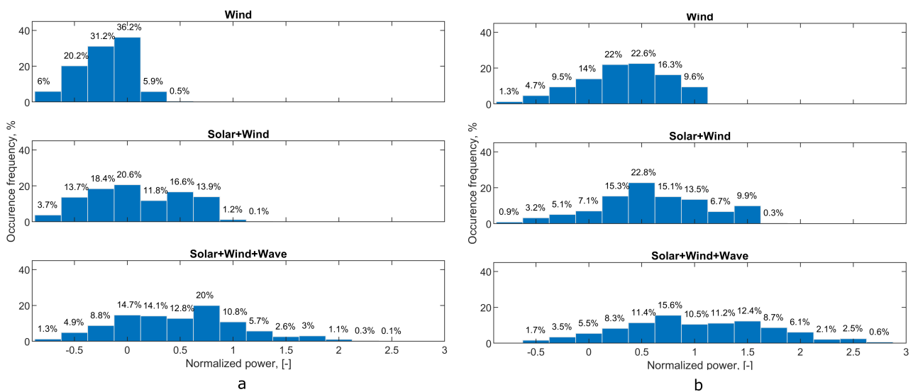
Figure 12. Occurrence frequency of net load during: (a) 1994; (b) 2007.
