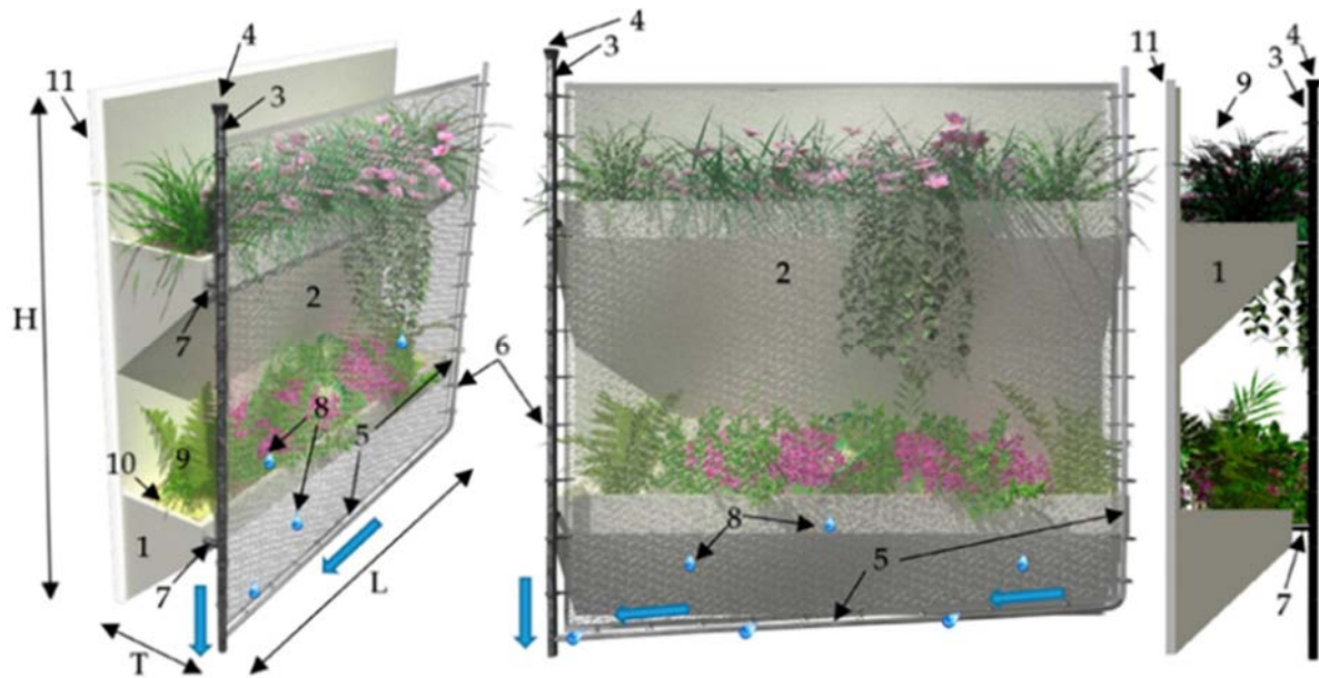
Figure 6. The innovative living wall platform incorporating a fog harvesting mesh is depicted as follows: 1—living wall platform, 2—fog harvesting mesh, 3—water collector pipe, 4—funnel connected to the collector pipe for water drop collection, 5—rod facilitating water drop conveyance to the collector pipe, 6—metal clamp securing the mesh to the pipe and rod, 7—support for affixing the mesh system to the green wall platform, 8—water droplets, 9—plants, 10—soil, 11—frame for securing the living wall to the building’s wall, H—height of the platform, L—length of the platform, T—thickness of the platform. Source: [23].
