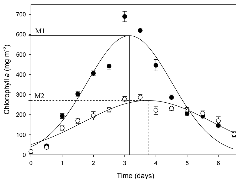
Figure 2. Variation of chlorophyll- a concentration in the phytoplankton batch culture with LED-on and -off conditions. A non-linear regression on daily triplicate measurements (solid circles indicate LED-on and open circles indicate LED-off) with a Gaussian model yielded the regression line (solid line). The maximum growth determined by the regression model was 593\text{ mg m}^{-3} at 3.1 days (M1, solid line) under the LED-on condition and 270\text{ mg m}^{-3} at 3.7 days (M2, dotted line) under the LED-off condition.
