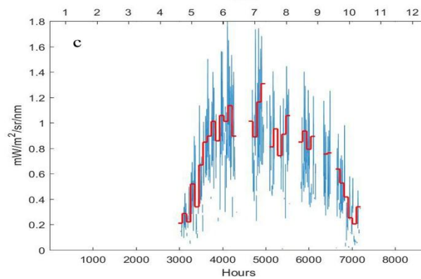
Figure 2. The time series of hourly (a) SIF 687 (mW/m 2 /sr/nm), (b) SIF 720 (mW/m 2 /sr/nm) and (c) SIF 761 (mW/m 2 /sr/nm) at the Harvard Forest site in 2014. The red lines represent 4-day daytime averages. The values in the top x-axes represent months.
