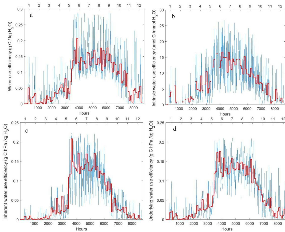
Figure 1. The time series of hourly (a) water use efficiency (WUE, g C/kg H 2 O); (b) intrinsic water use efficiency (WUE i , umol C /mmol H 2 O); (c) inherent water use efficiency (IWUE, g C hPa /kg H 2 O) and (d) underlying water use efficiency (uWUE, g C hPa /kg H 2 O) at the Harvard Forest site in 2014. The red lines represent 4-day daytime averages. The values in the top x-axes represent months.
