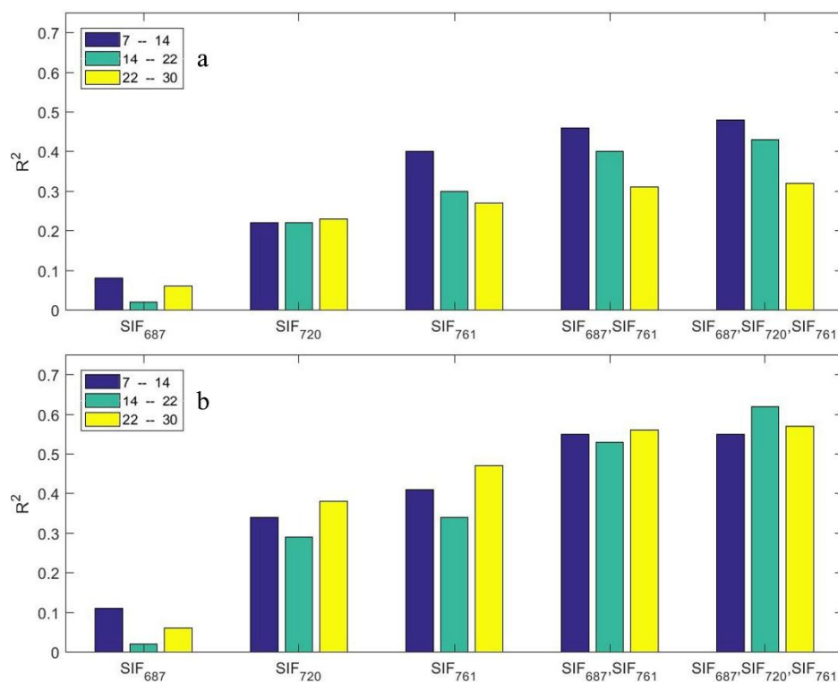
Figure 5. The effect of air temperature ( T_{\text{air}} , °C) on the coefficients of determination ( R^2 ) between IWUE and the selected single SIF bands and their combinations by using (a) linear regression analysis and (b) Gaussian processes regression, respectively. The blue, green and yellow bars represent R^2 from data with T_{\text{air}} \leq 14 °C, 14 °C < T_{\text{air}} < 22 °C, and T_{\text{air}} \geq 22 °C, respectively. All data have an hourly time resolution and belong to the period between 7 a.m. and 5 p.m. local time.
