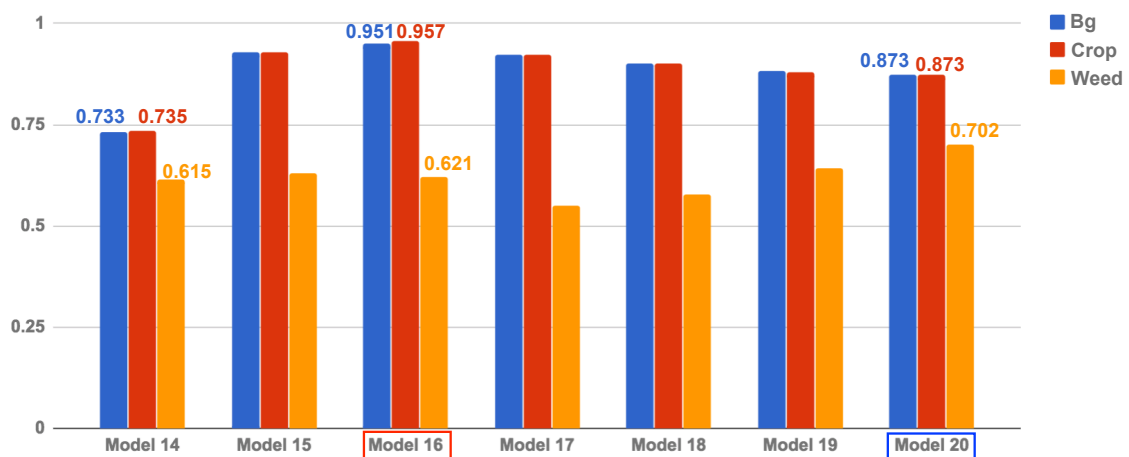
Figure 11. Quantitative evaluation of the segmentation using area under the curve (AUC) of the Sequoia dataset. As in the RedEdge-M dataset, the red box indicates the best model, and the blue box is a model with only one NDVI image input.
