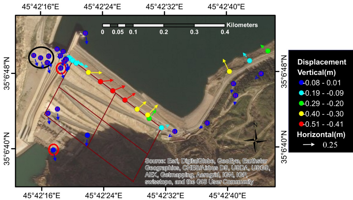
Figure S2. The horizontal (indicated by arrows) and vertical (indicated by circles) displacements of the monitoring pillars on Derbandkhan dam measured by GPS and levelling. The source of the background image is from [16]. Note that (i) the horizontal displacements are referenced to ITRF08, and (ii) the pillars labelled with letter H were measured with GPS only.
