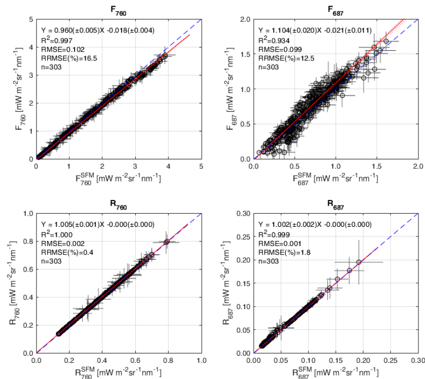
Figure 11. Scatterplot between fluorescence (top) and reflectance (bottom) at 760 nm (left) and 687 nm (right) estimated by SFM and the novel F spectrum algorithm. The dots represent hourly average values (standard deviation) for the entire time series acquired on different crops during the entire season. The red line is the OLS linear regression model; dashed blue line the 1:1.
