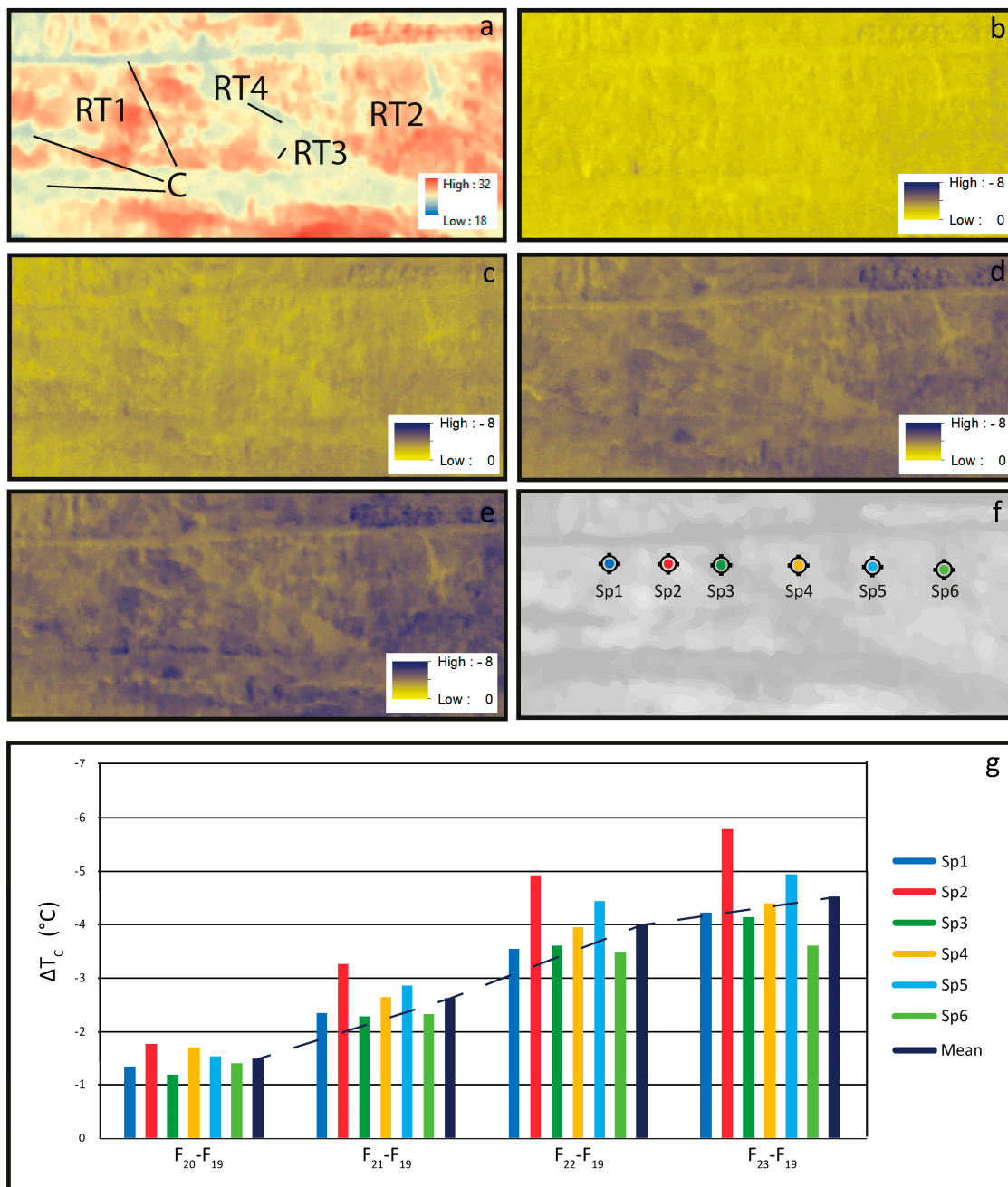
Figure 10. Summer measurement session (a) = image at 19:00 ( F_{19} ), (b) = F_{20}-F_{19} , (c) = F_{21}-F_{19} , (d) = F_{22}-F_{19} , (e) = F_{23}-F_{19} , (f) = position of measurement points, and (g) = temperature differentials of the spot measurement points.
