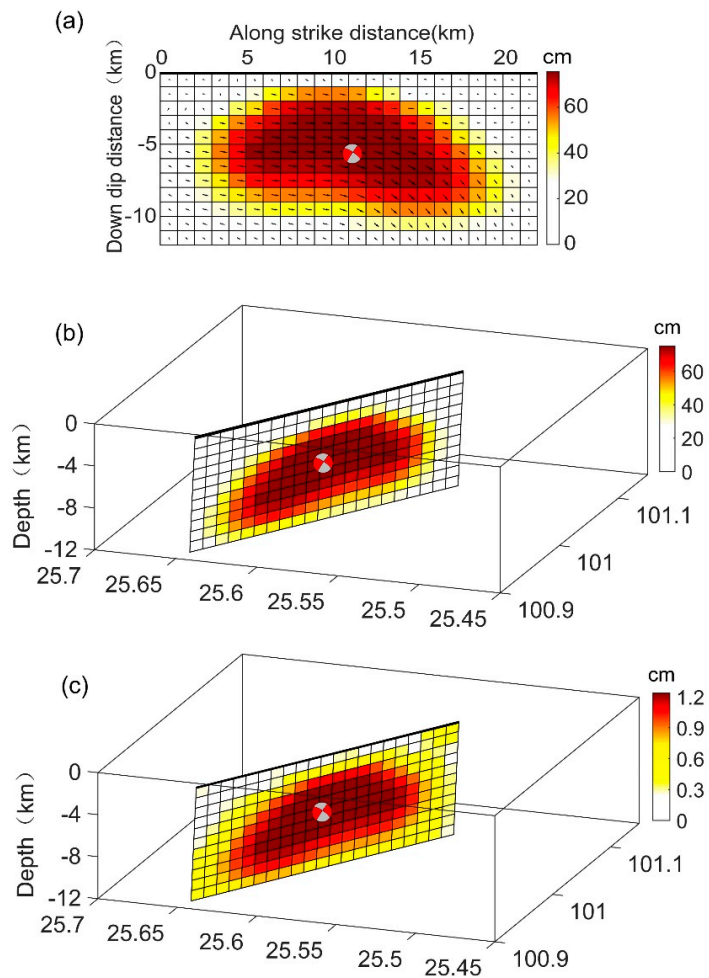
Figure 6. (a) Slip distributions for a fault plane of 22 km length, 12 km downdip width, and 87° dip; (b) 3-D view of the fault from WSW; (c) 1σ uncertainty in fault slip estimated through a Monte Carlo process with 100 inversions. The thick black line in the top of each subfigure represent the projection of fault trace on the surface.
