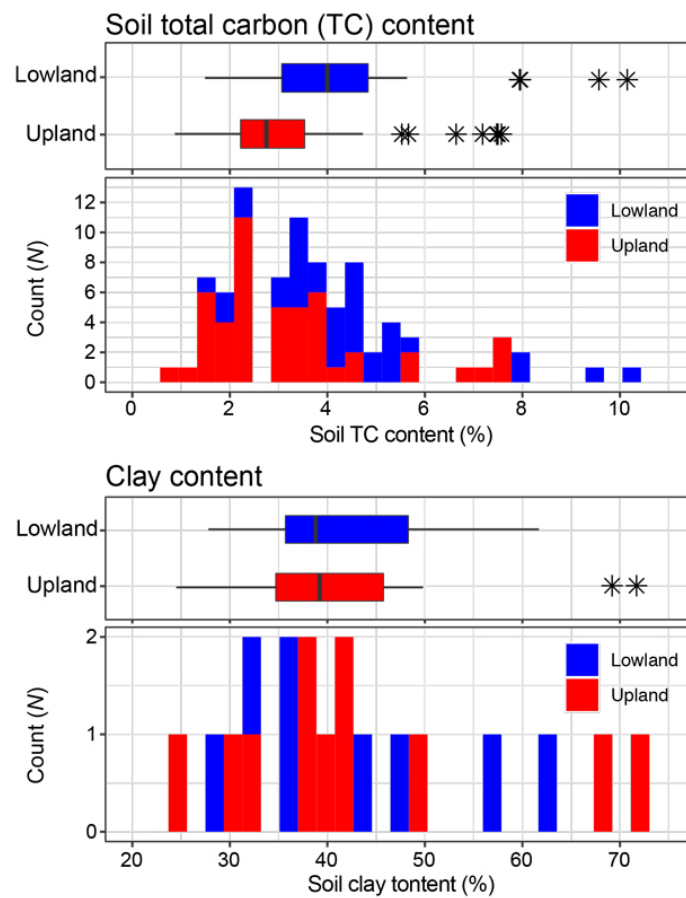
SI: Figure S1. Box plot and histogram of soil total carbon (TC) and clay contents in the lowland and upland data sets.
