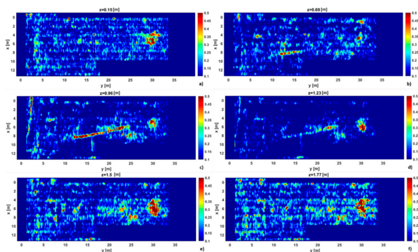
Figure 4. Visualization of the pseudo-3D GPR tomographic results by means of slices at different depths: (a) 0.15 m; (b) 0.69 m; (c) 0.96 m; (d) 1.23 m; (e) 1.5 m; (f) 1.77 m. Several anomalies are visible, which are ascribed to the presence of duct and cisterns for water storage. The tomographic images show the normalized intensity of the obtained contrast.
