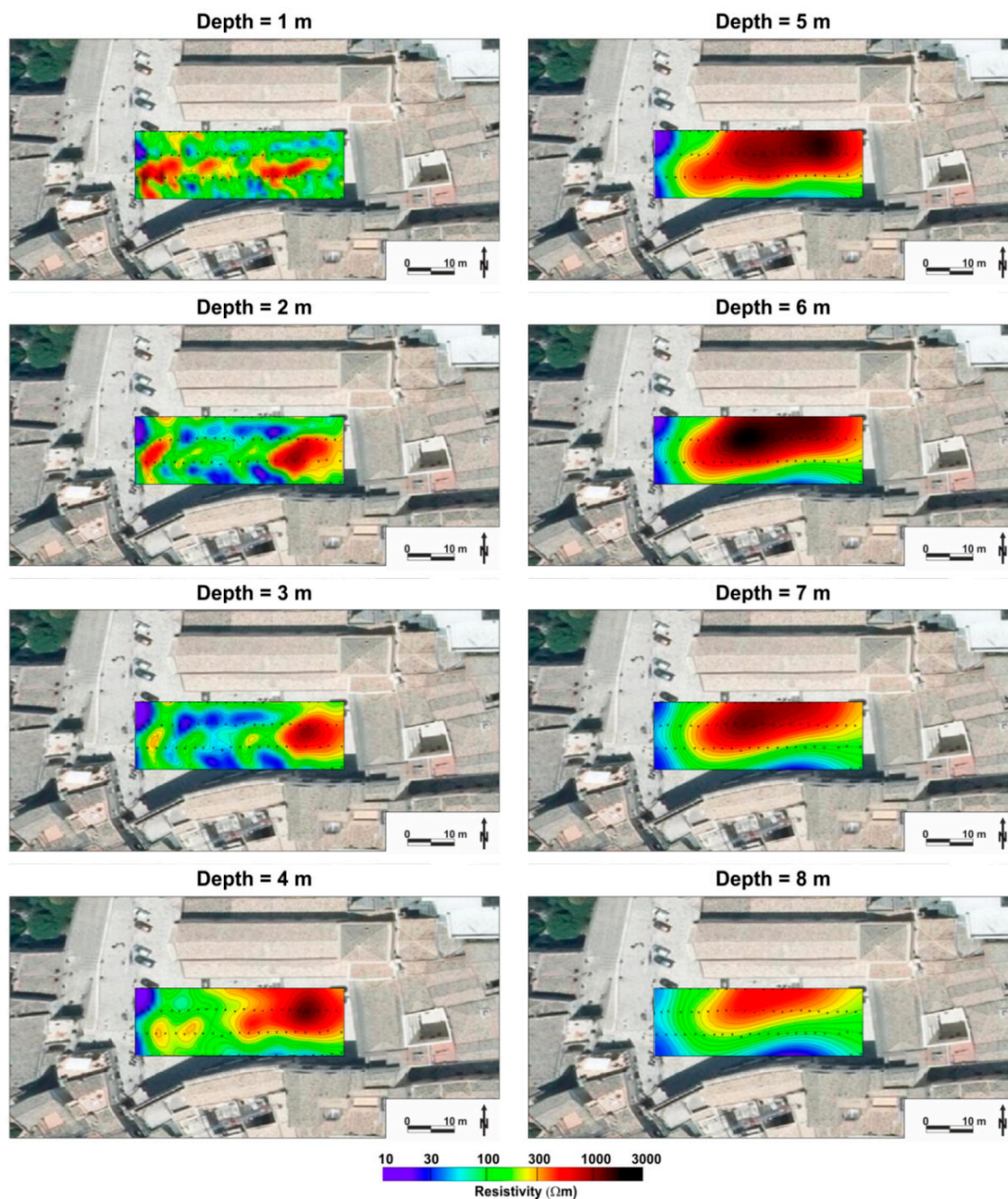
Figure 7. Results of the 3D ERT tomographic images represented by means of constant depth slices (Image modified from Google Earth).
