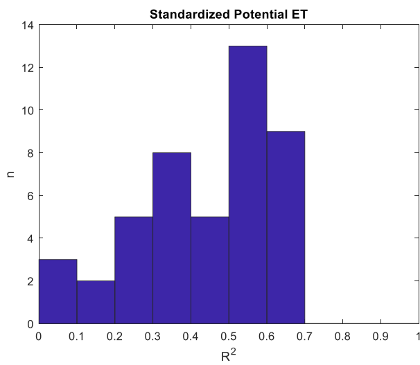
Figure S1. Comparison of coefficients of determination ( R^2 ) histograms for NDVI relations to Standardized Precipitation-Evapotranspiration Index (SPEI), Standardized Precipitation, and Standardized Potential Evapotranspiration by EPA Level 4 Ecoregion.
