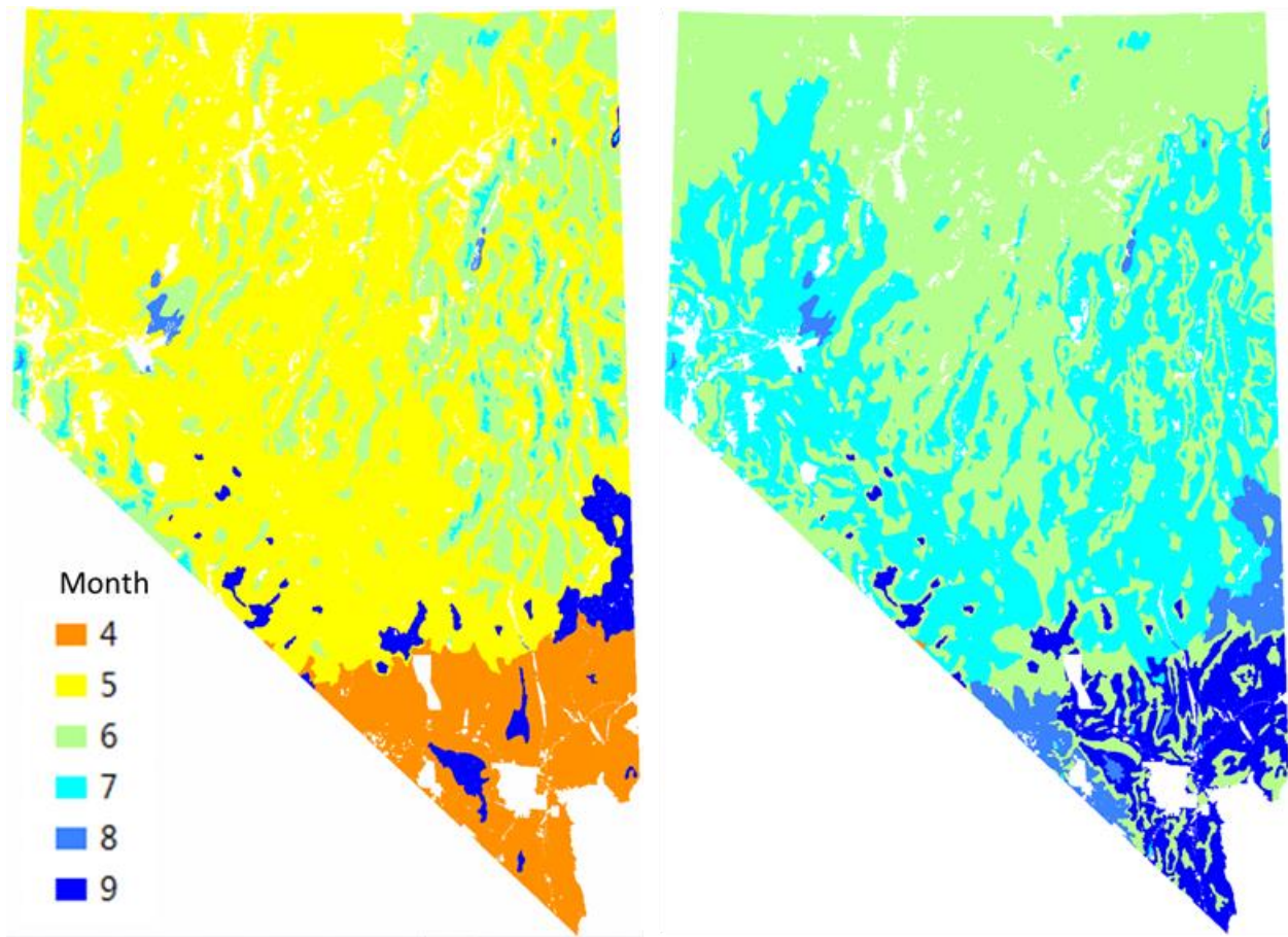
Figure S2. Month of peak NDVI in upland (left) and riparian (right) vegetation by EPA Level 4 Ecoregion.
