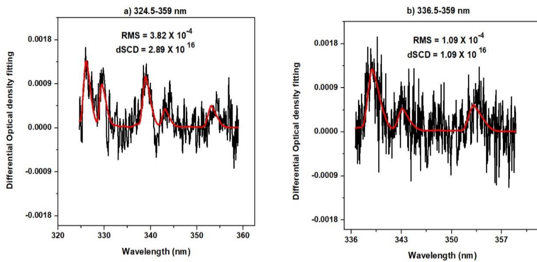
Figure 3. HCHO DOAS fit for fitting window (a) 324.5–359 nm and (b) 336.5–359 nm at 2^\circ elevation angle. The red lines represent the fitted optical density, while measured densities are shown by the black lines.
