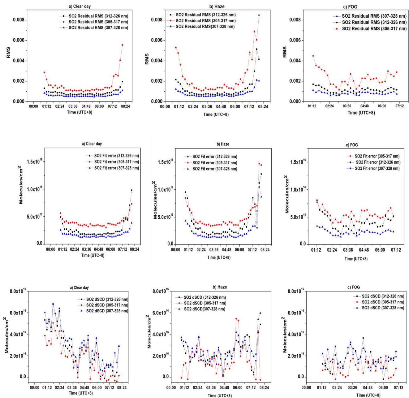
Figure 7. Intercomparison of different retrieval settings by parameters such as DOAS fit error, RMS, and SO 2 DSCDs on a (a) clear day (17 February 2020), (b) hazy day (31 January 2020), and (c) foggy day (13 February 2020).
