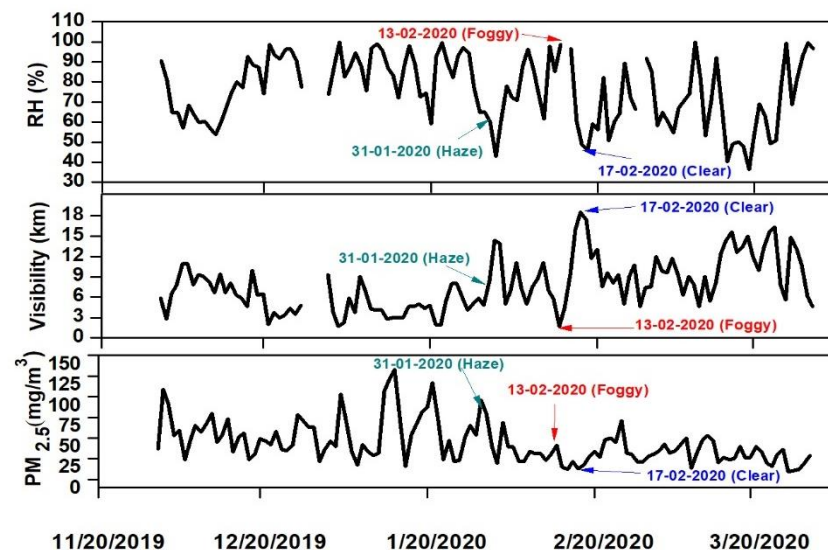
Figure 2. Time series for relative humidity (RH%), visibility, and \text{PM}_{2.5} .
