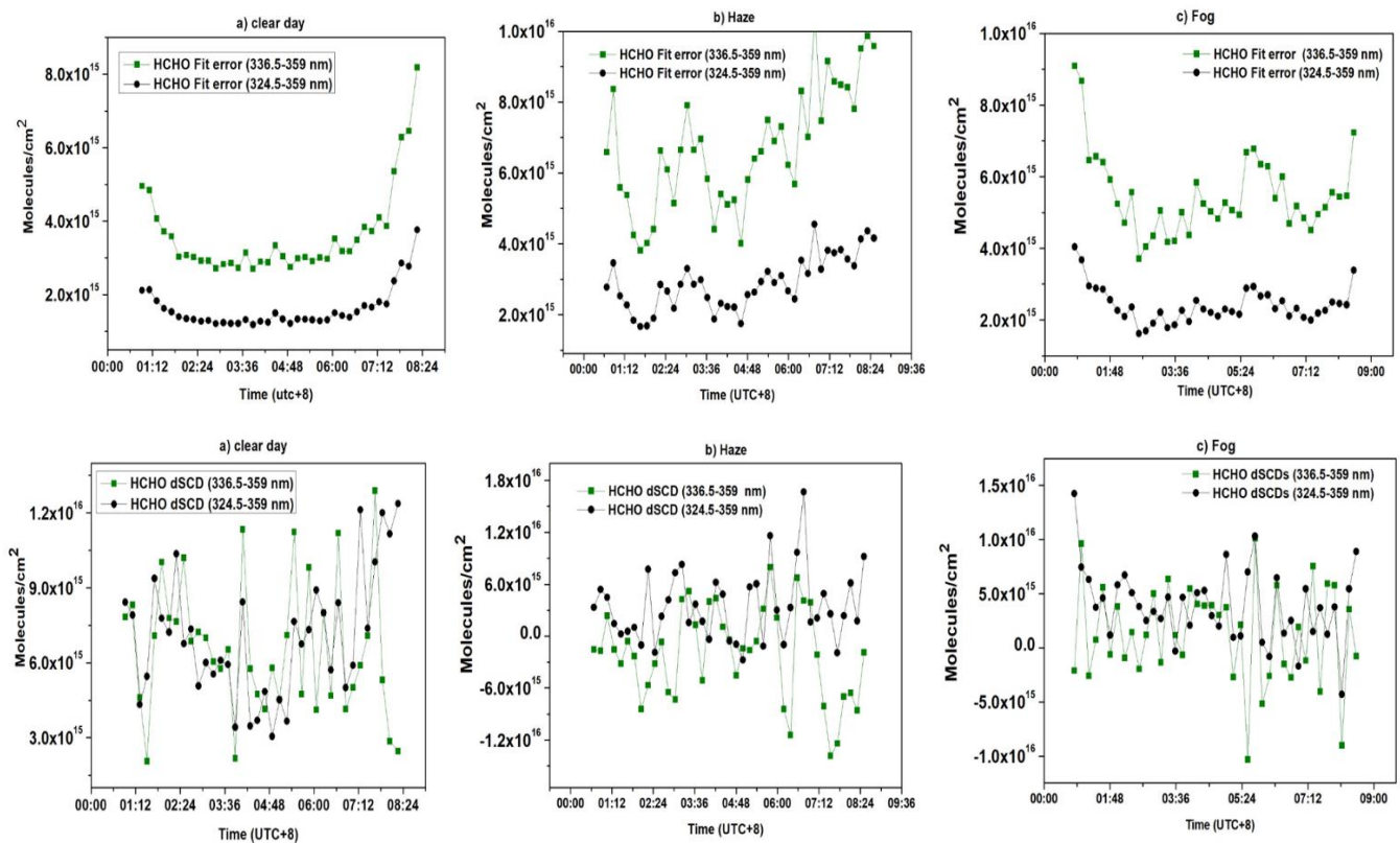
Figure 4. Intercomparison of different retrieval settings by parameters like DOAS fit error, RMS, and HCHO DSCDs for a) clear day (17 February 2020), b) hazy day (31 January 2020), and c) foggy day (13 February 2020).
