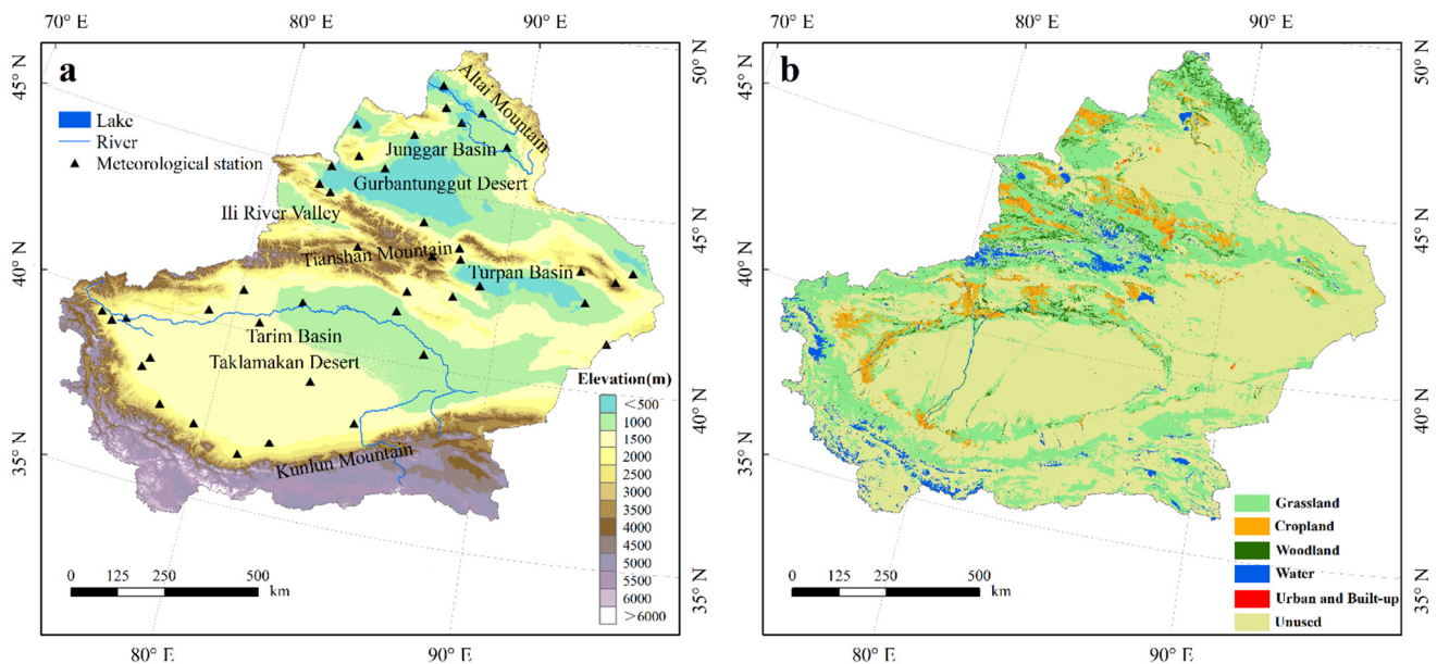
Figure 1. (a) Meteorological stations in Xinjiang overlaid on the terrain map (Shuttle Radar Topography Mission; https://eosps.gsf.nasa.gov/missions/shuttle-radar-topography-mission , accessed on 8 February 2021). (b) Land use types in 2010 in Xinjiang ( http://www.resdc.cn/ , accessed on 2 March 2021).
