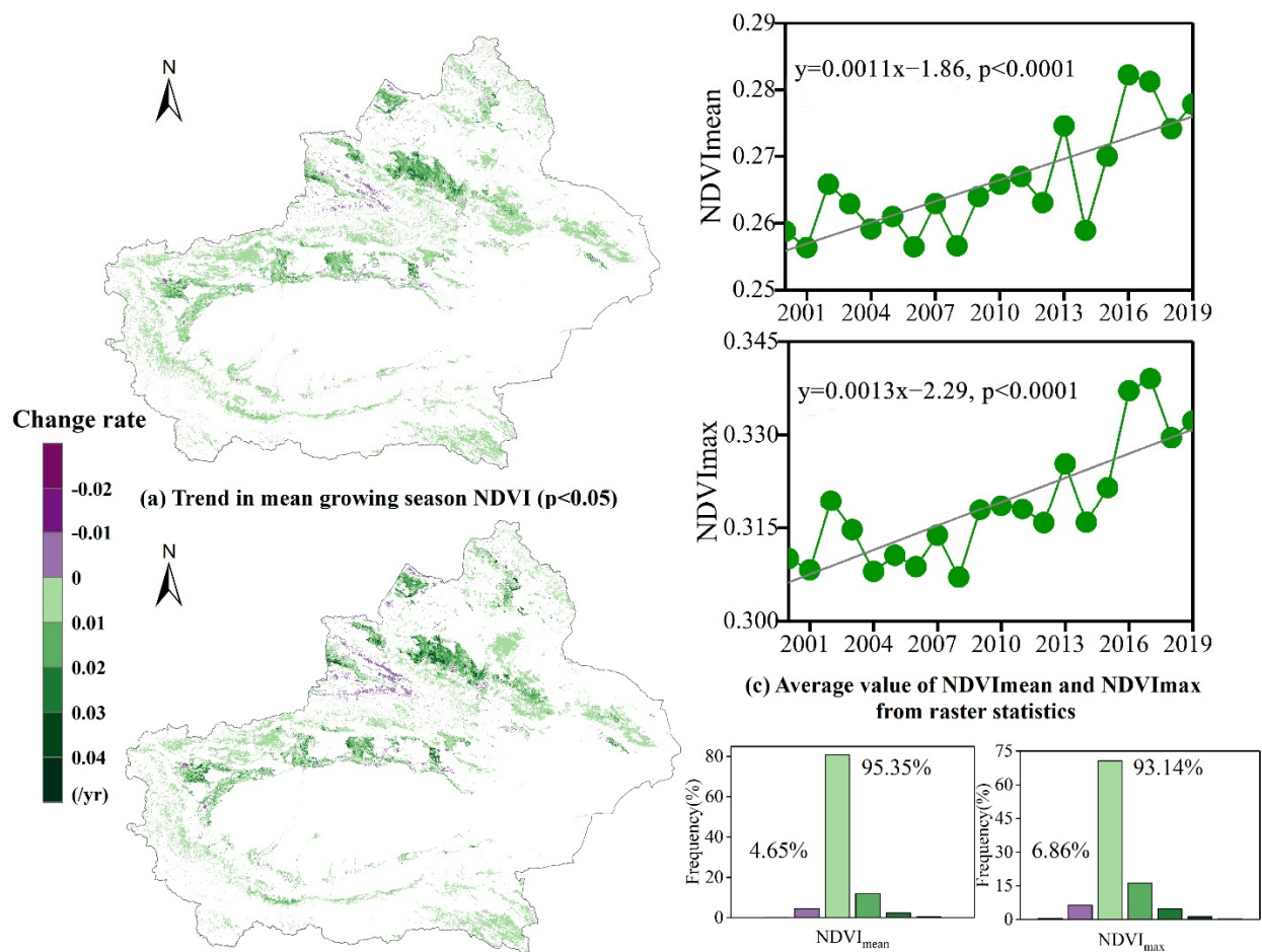
Figure 3. The spatial patterns of (a) change rate of mean NDVI ( R_{\text{mean}} ) for 2000–2019 and (b) change rate of maximum NDVI ( R_{\text{max}} ) for 2000–2019. The white parts indicate the areas where the multiyear \text{NDVI}_{\text{mean}} is under 0.1. (c) The long-term trend of \text{NDVI}_{\text{mean}} and \text{NDVI}_{\text{max}} for 2000–2019 based on the average value from zonal raster statistics. (d) The frequency of \text{NDVI}_{\text{mean}} and \text{NDVI}_{\text{max}} change rate for different numerical intervals. The NDVI was calculated throughout the growing season (May to September).
