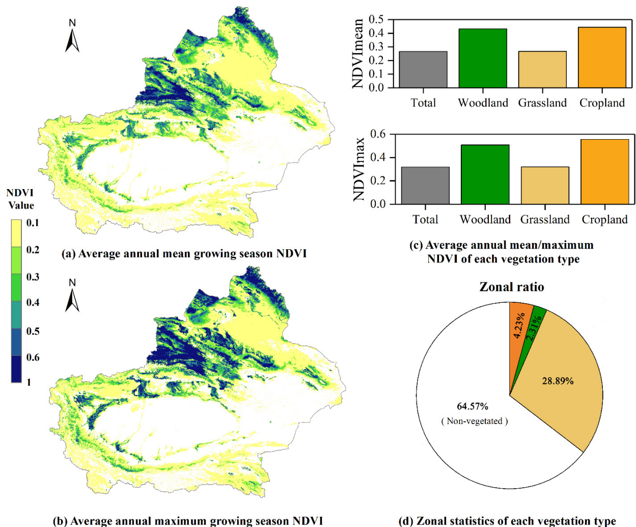
Figure 2. Spatial patterns of the long-term average growing season NDVI for 2000–2019, (a) mean NDVI (NDVI mean ), (b) maximum NDVI (NDVI max ). The white parts indicate the areas where the multiyear NDVI mean is under 0.1. (c) Average annual NDVI mean and NDVI max of each land use type for 2000–2019. The NDVI was calculated for the growing season from May to September. (d) Zonal statistics for each land use type were based on the land use map.
