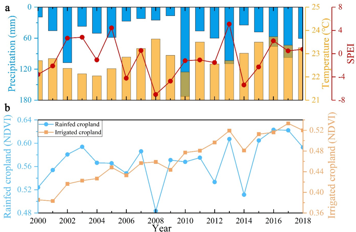
Figure 9. Long-term growing season (May–September) trend of (a) total precipitation, and average mean temperature and SPEI that spatially aggregated over cropland, (b) the average NDVI mean of the grid cells for rain-fed and irrigated cropland.
