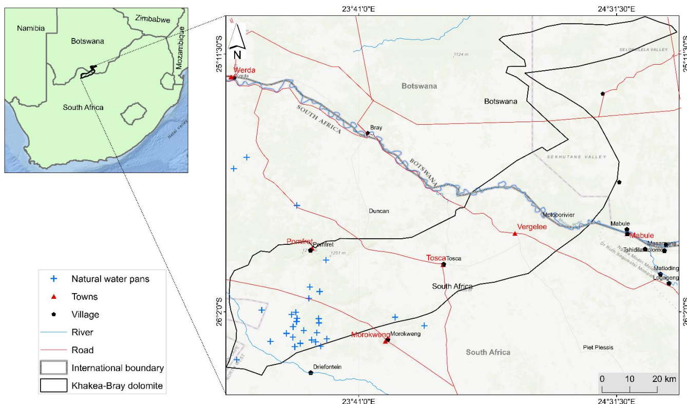
Figure 1. Map of the Khakea-Bray TBA spanning across Botswana and South Africa. The study is overlaid on baseline topography imagery accessed from ArcMap [49].
