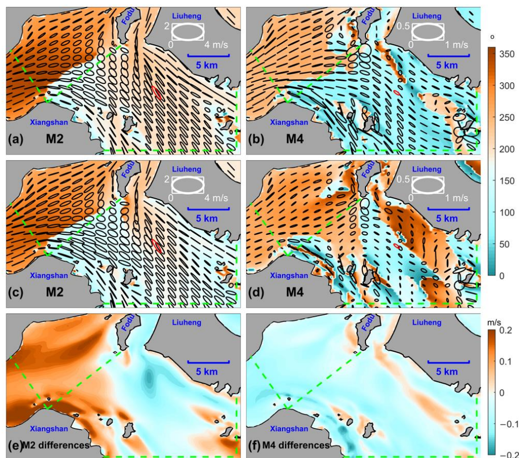
Figure 10. Distributions of vertical-averaged tidal current ellipses (black ellipses, in m/s) and phases (contour plots, in ^{\circ} ) that were obtained by (a,b) Case3 and (c,d) Case0 models. The red ellipses were obtained by ADCP data. The tidal constituents are presented in the bottom left of each panel. The scale of tidal current ellipses of M2 and M4 are plotted in the upper-right corner of each panel. The distributions of amplitude differences for (e) M2 and (f) M4 between Case3 and Case0 (in m/s). Positive values indicate Case0 > Case3.
