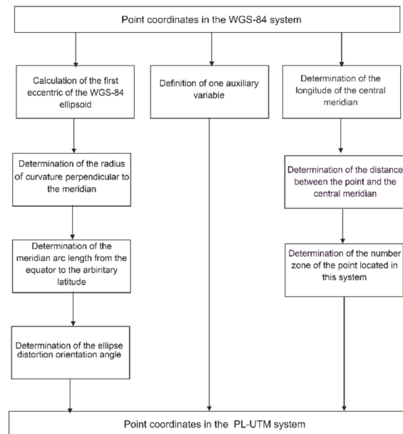
Figure 2. Flowchart showing steps of model for the transformation ellipsoidal coordinates to plane coordinates in the PL–UTM system.
