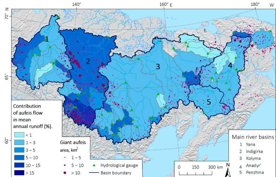
Figure 6. Contribution of aufeis flow in mean annual river runoff (%).
