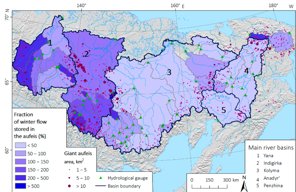
Figure 7. The fraction of winter flow stored in the aufeis (%).
