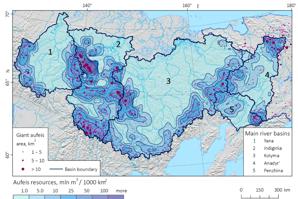
Figure 4. Aufeis resources of the North-Eastern Eurasia.
