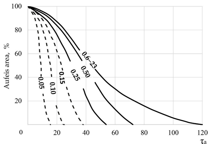
Figure 2. The aufeis area decrease during the warm period of the year, depending on the number of days ( \tau_a ) after the start of ablation, and their maximum area (The numbers at the curves, km 2 ) adopted from [34]. Solid and dotted lines present the dependencies derived from observed data (solid) and extrapolated.
