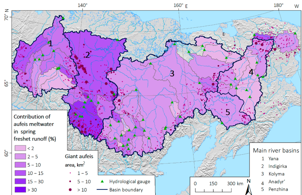
Figure 8. Contribution of aufeis meltwater in spring freshet runoff (%).
