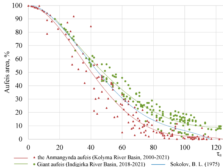
Figure 3. The comparison of the historical curve 0.6–23 by Sokolov (1975) [38] and recent aufeis area data in the Indigirka and the Kolyma River basins (2000–2021).
