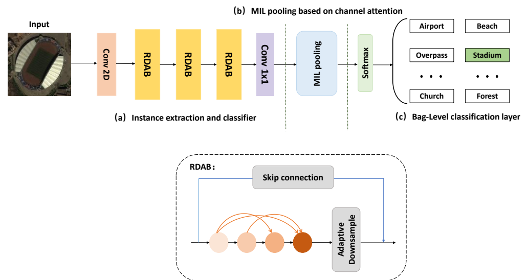
Figure 3. Overall structure of the proposed MILRDA model. The model consists of three parts: (a) instance extraction and classifier, (b) MIL pooling based on channel attention and (c) bag-level classification layer.
