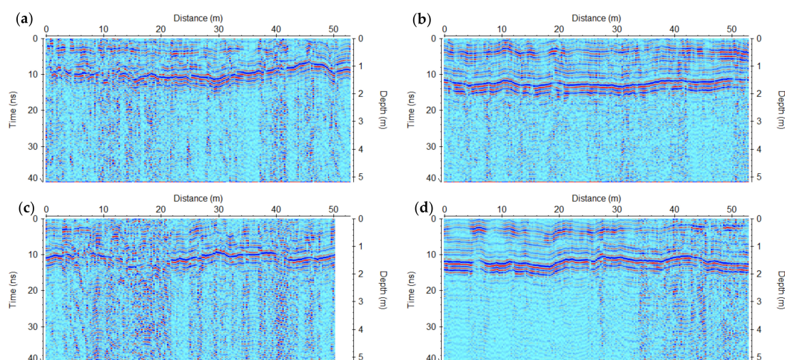
Figure 13. Four parallel sections of the Gressoney test sites after subtracting the flight altitude (letters (a–d) correspond to the 4 GPR sections indicated in the bottom left of Figure 5).
