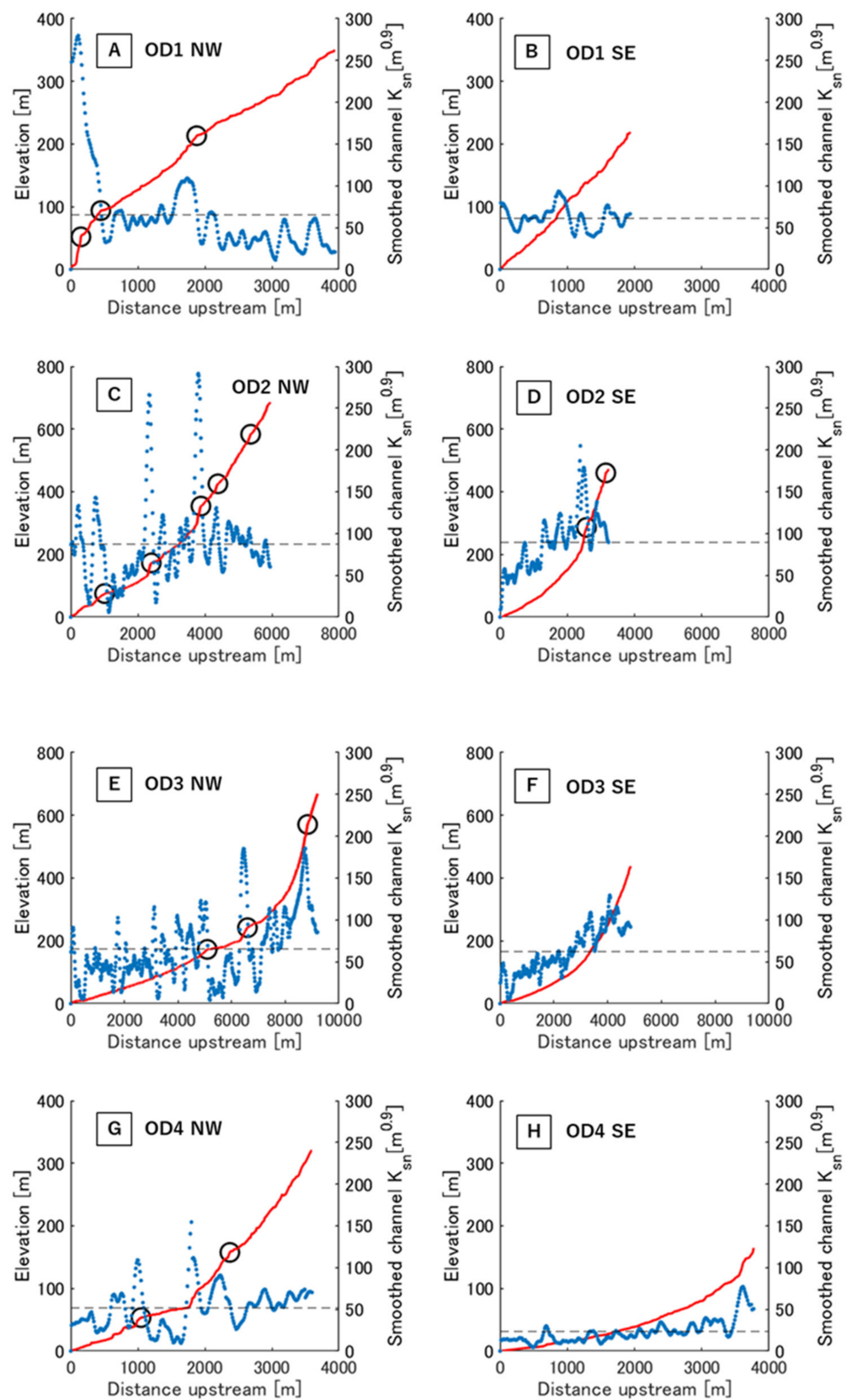
Figure 5. Representative river profiles (red lines) and knickpoints (black circles) for each analysis segment (OD1–4) in Osado, in addition to the k_{sn} values (blue dots). Representative channels used in the calculations are shown in Figure 3. NW and SE indicate the northwestern and southeastern sides of the divide, respectively. The channels were chosen to avoid those that include the Kuninaka Plain to eliminate the effects of sedimentation, and those that have not been developed with dam construction.
