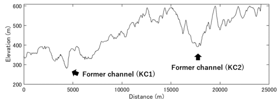
Figure 17. Elevation profile along the divide. The depressions indicated by arrows represent a region in the middle of the abandoned channels as shown in Figure 15 (dotted lines) and correspond to the cross-sections of former channels prior to stream capture.
