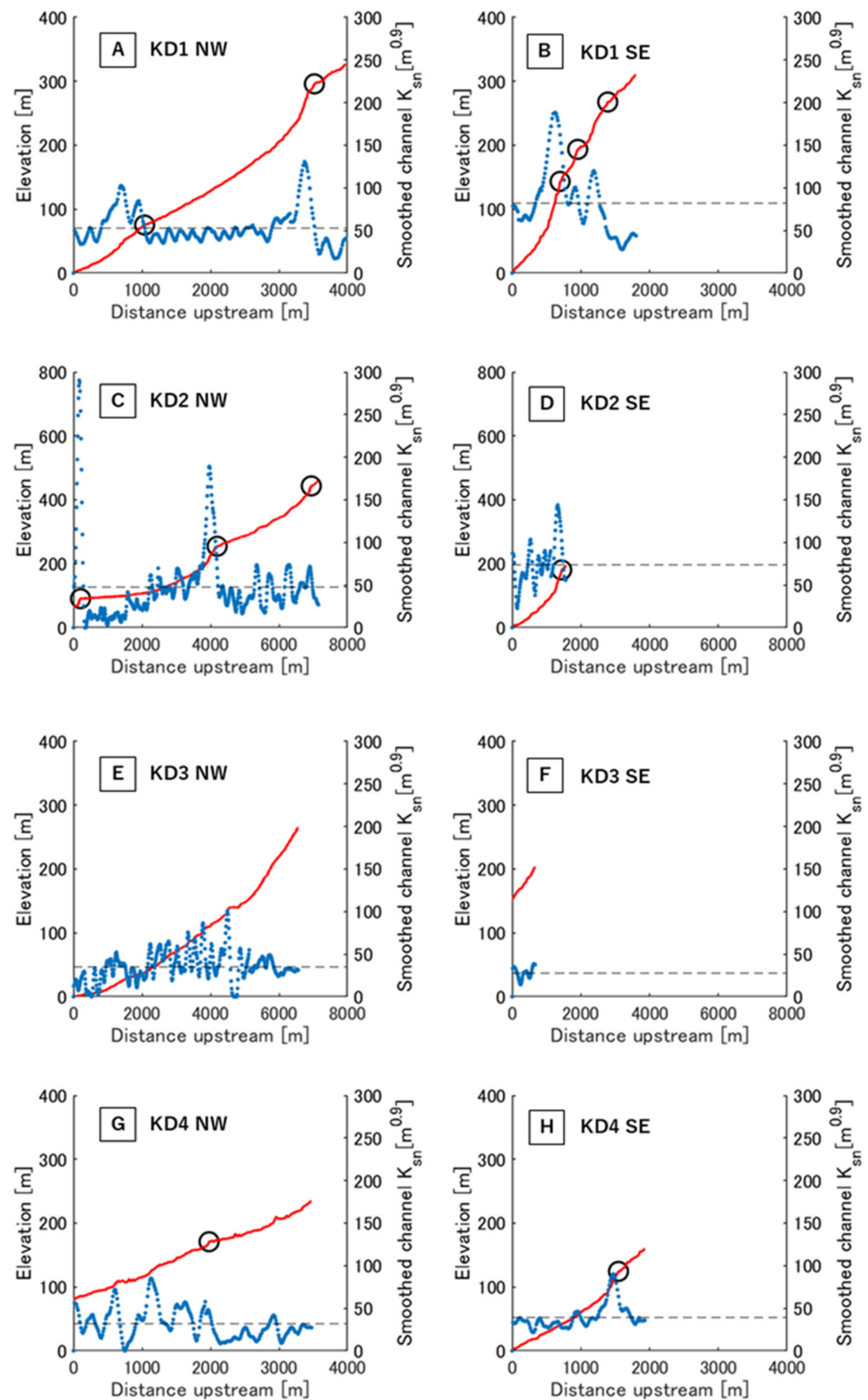
Figure 6. Representative river profiles (red lines) and knickpoints (black circles) for each segment in Kosado, in addition to the k_{sn} values (blue dots). Representative channels used in the calculations are shown in Figure 4. NW and SE indicate the northwestern and southeastern sides of the divide, respectively. KD2 in (C) represents channels above 70 m in elevation to avoid the influence of plains. Rivers in (F,G) are both tributaries of the Hamo River, and shown upstream of confluences. The channels were chosen to avoid those that include the Kuninaka Plain to eliminate the effects of sedimentation, and those that have not been developed with dam construction.
