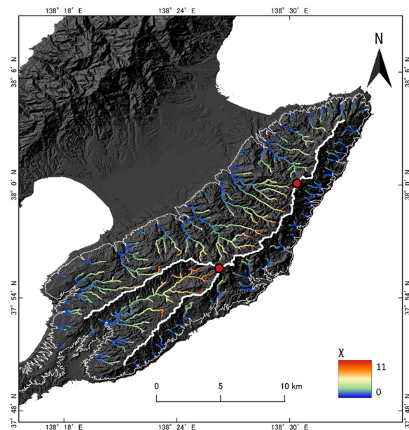
Figure 11. \chi map for Kosado, where the base-level was set to 70 m in elevation, to avoid the effects of alluvial plains. The thin white line indicates an elevation of 70 m, whereas thick white line is the main divide of Kosado.
