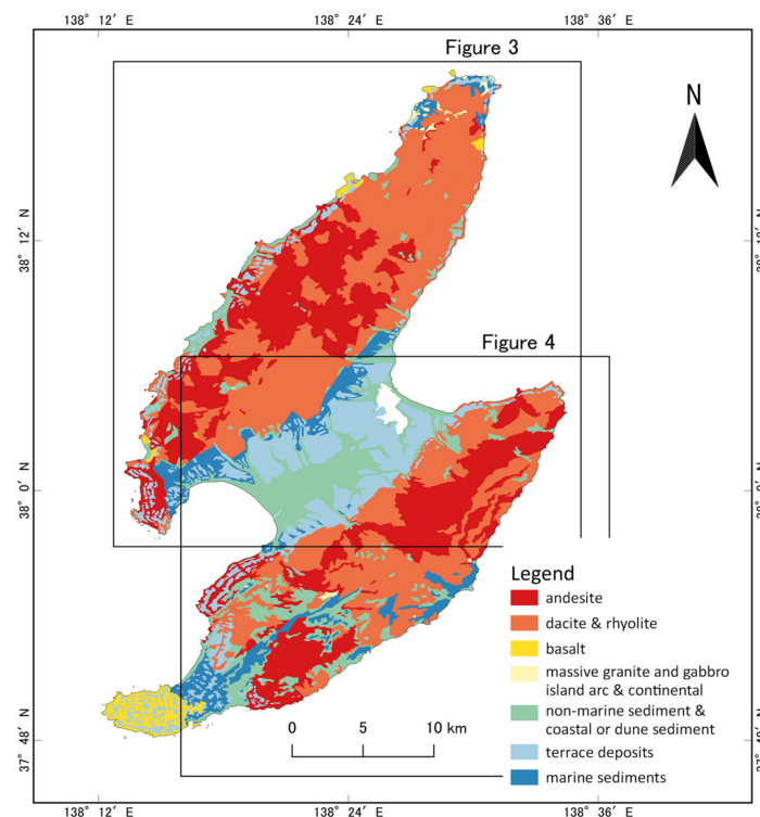
Figure 2. Geological map of Sado Island. This map follows the Seamless Geological Map of Japan 1:200,000 V2 (Geological Survey of Japan, AIST, Data updated on 6 April 2020, https://gbank.gsj.jp/seamless/ , accessed on 22 October 2021) Revised. The two rectangles indicate the locations of Figures 3 and 4.
