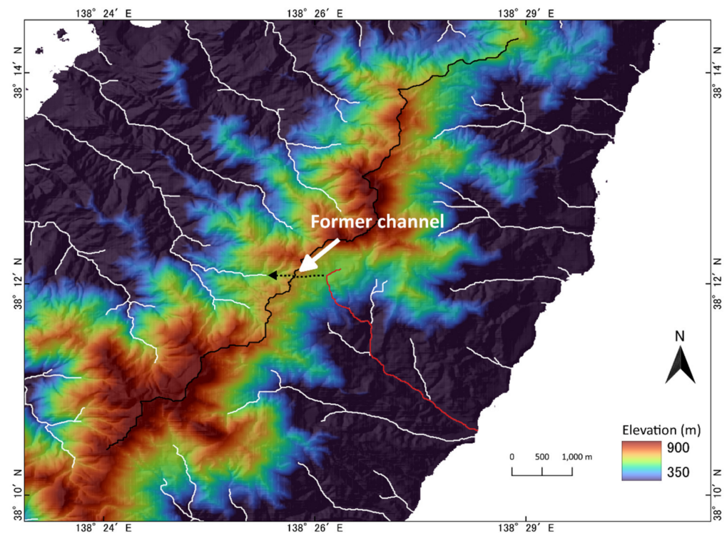
Figure 12. Location of past river capture in Osado. The red line is the GISmap conforming river, possessing a sharp bend, that pirated the upstream reach from a river flowing on the northwestern side. The black dotted line with arrow indicates the location and flow direction of the abandoned channel, where it was connected to the front edge of the bend.
