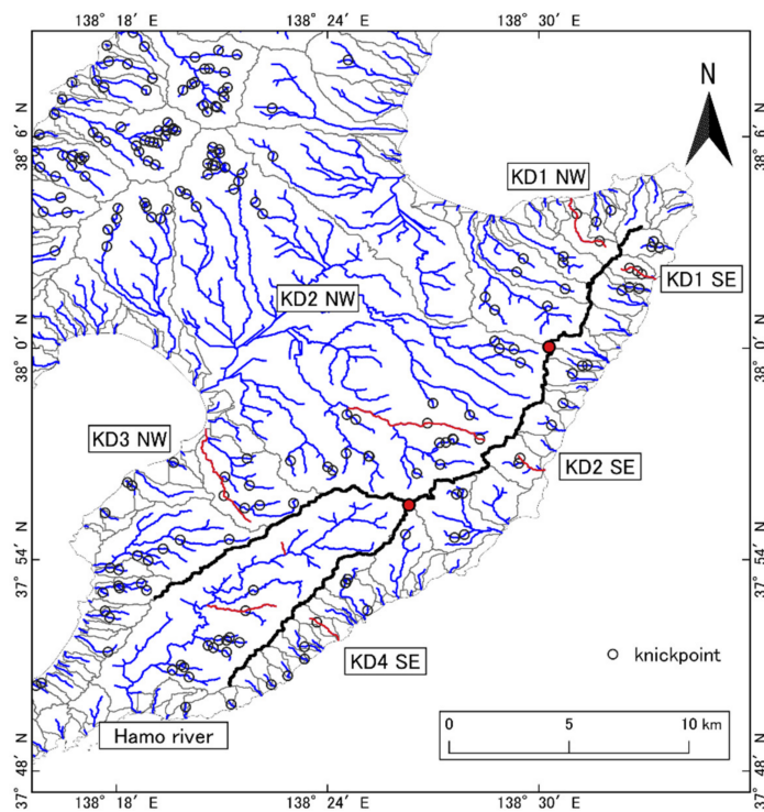
Figure 4. Location of stream channels and knickpoints in Kosado. Blue and red lines exhibit stream channels. Black circles represent the location of knickpoints. The red channels are representative channels in each segment.
