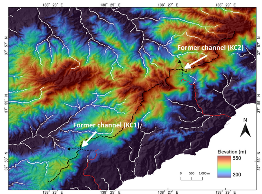
Figure 15. Locations of past river capture in Kosado. The red lines are the GSI map conforming rivers that captured the upstream reach from a river flowing toward northwest; and thus, had a sharp bend in the upstream reach. The black dotted lines with arrows indicate the locations and flow directions of the abandoned channels where they used to be connected to the bend reaches.
