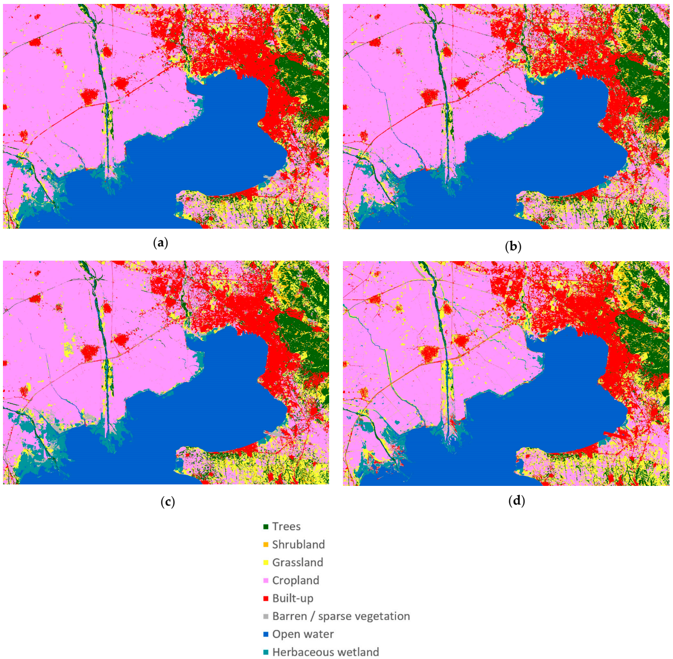
Figure 8. The predicted segmentation maps for each method. From left to right, top to bottom: (a) SegFormer B0, (b) SegFormer B5, (c) U-NET, and (d) U-TAE.
