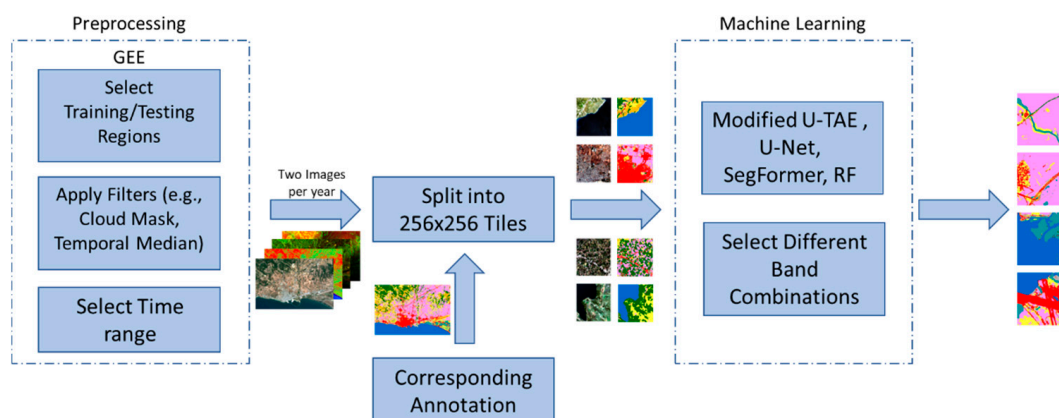
Figure 1. Flowchart of the proposed land cover classification approach.
