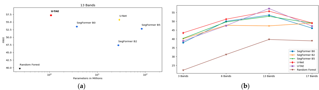
Figure 5. (a) The mIoU score for each model in regard to its parameters. (b) The effect of band input on each model's mIoU score. The highest overall result is achieved by U-TAE.
