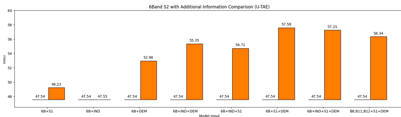
Figure 10. mIoU scores for U-TAE models using different band combinations. At the left of each bar, the mIoU score resulting from the U-TAE model for the 6B band configuration is presented as a baseline.
