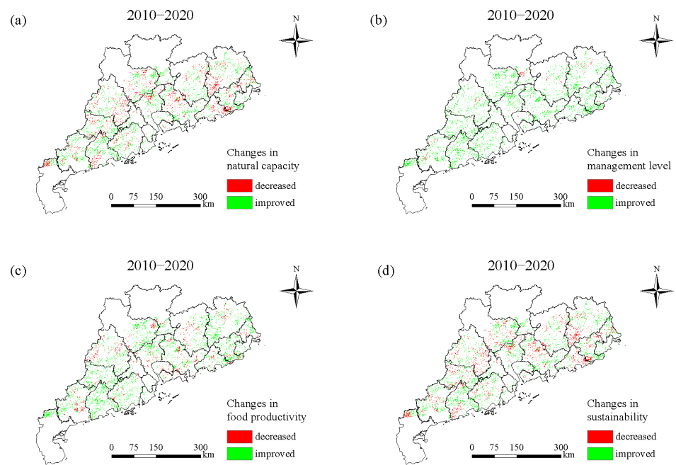
Figure 5. Dynamic changes in natural capacity (a), management level (b), food productivity (c), and cropland sustainability (d) from 2010 to 2020.
