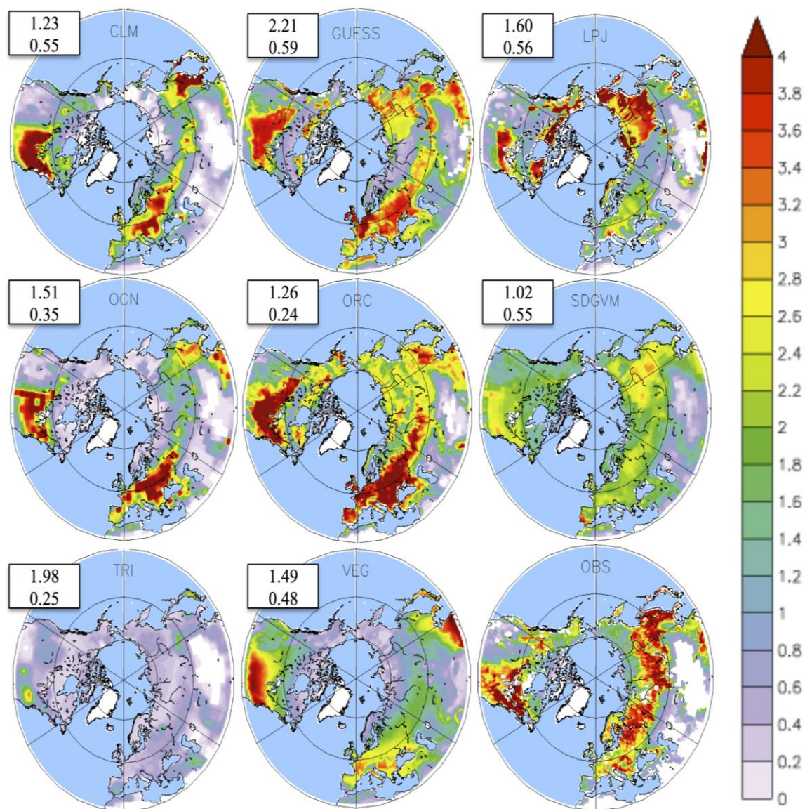
Figure 4. Seasonal Amplitude in LAI for 8 LSMs and satellite observations for the Northern Hemisphere (30°–90° N) for the period 1986–2005. Root mean square errors and spatial correlations between each model and the observations are given in the white boxes.
