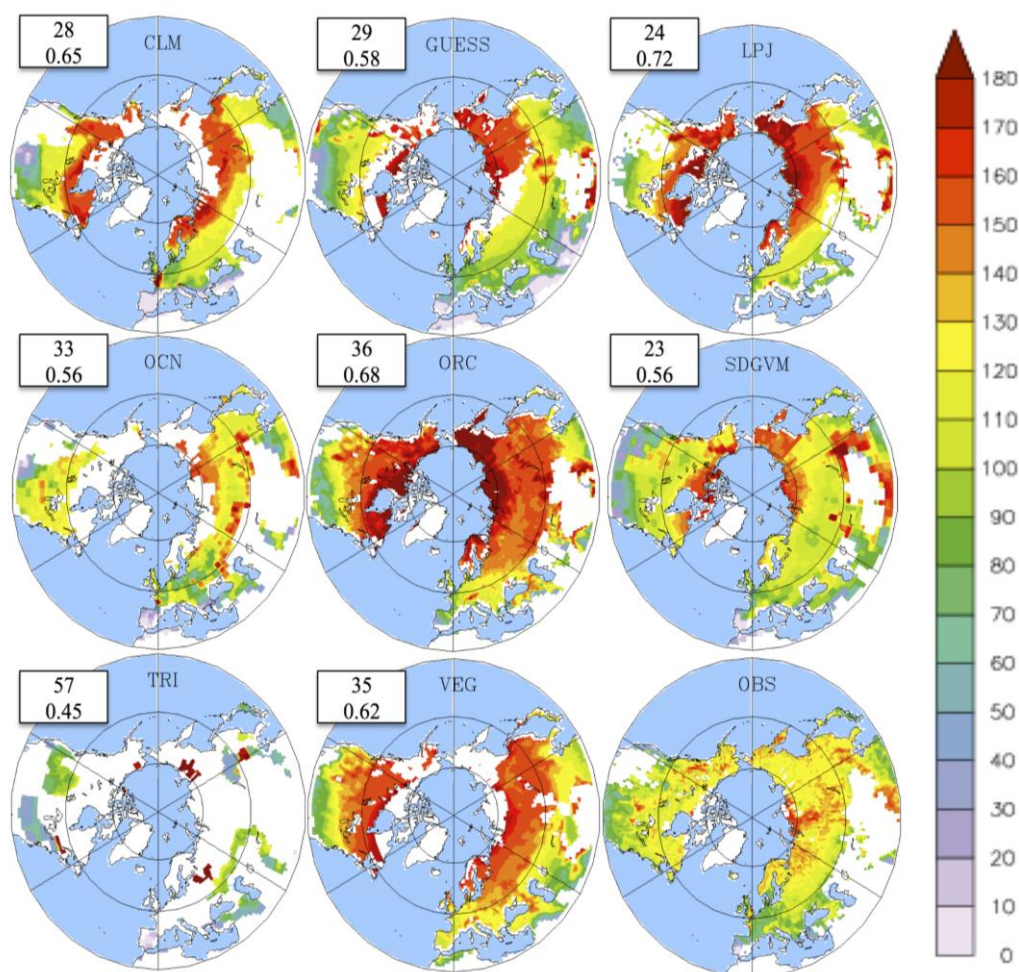
Figure 5. Mean (1986–2005) growing season onset (day) for 8 LSMs and satellite observations over the Northern Hemisphere (30 °–90 °N). Spatial correlations and root mean square errors between each model and the observations are given in the white boxes.
