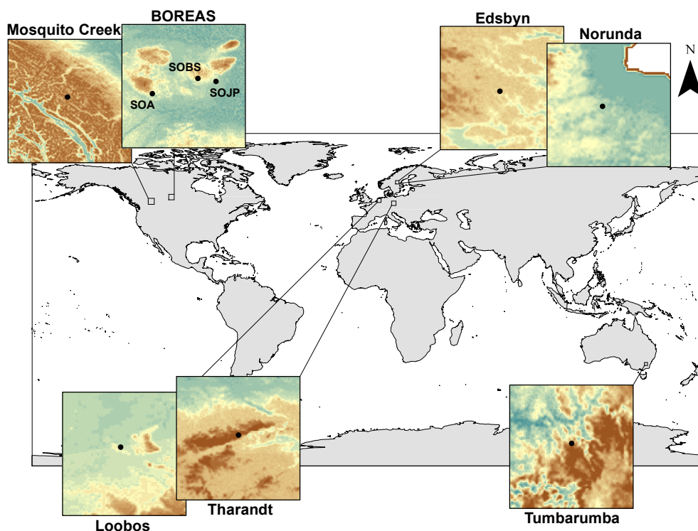
Figure 2. Map of all sites employed in this study. Local relief at each site is illustrated in respective panes (source: Natural Earth). Note: each panel highlights broad-scale terrain characteristics at each site, and as a result, elevation range varies with site; sit-specific elevation ranges are given in Table 3.
