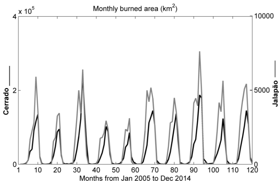
Figure 8. Monthly burned area (km 2 ) for the 10-year period over Cerrado (black curve) and Jalapão (gray curve).
