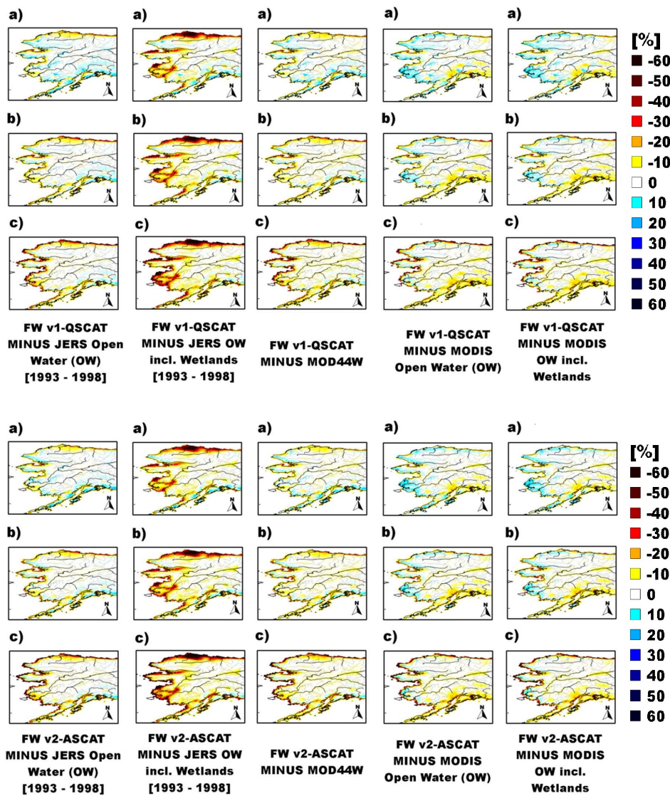
Figure 9. Difference maps between fractional water (FW) from v1-QSCAT (2000–2008) and v2-ASCAT (2009–2012) generated from (a) average annual maximum (FW max ); (b) mean (FW ave ); and (c) minimum (FW min ) minus open water (OW) and wetlands derived from the L-band Japanese Earth Resources Satellite (JERS)-based Alaska wetland map and subsets of static FW from the MOD44W and MODIS including wetlands products over the state of Alaska (54°N–72°N, 143°W–170°W). Actual figure color is a linear interpolation of the colors in the legend. Map projection same as Figure 2. Distance covered by one degree of latitude is approximately 111-km.
