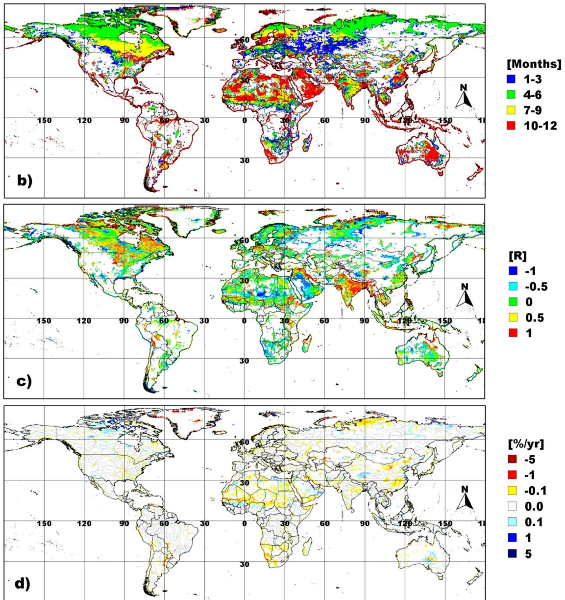
Figure 6. Global maps of: (a) the month of average maximum fractional water (FW); (b) the average number of inundated months; (c) the temporal linear correlation (R) between FW and the Modern-Era Retrospective Analysis for Research and Application (MERRA) precipitation analysis and (d) the trend of the annual FW means over the global domain as determine from combined, v1-ERS (1992–1999) and v1-QSCAT (2000–2008) monthly means and total monthly precipitation from the MERRA reanalysis (1992–2008). Actual figure color (c,d) is a linear interpolation of the colors in the legend. Except for (d), areas in white are outside of the domain or are screened (annual mean FW < 1%) from the analysis, while areas in dark grey represent snow covered regions. The annual FW trend was approximated from the slope of the least-square best fit-line and trend significance was assessed at a minimum 95% ( p < 0.05 ) probability level. Only statically significant trends are shown. Map projection same as Figure 2. Distance covered by one degree of latitude is approximately 111-km.
