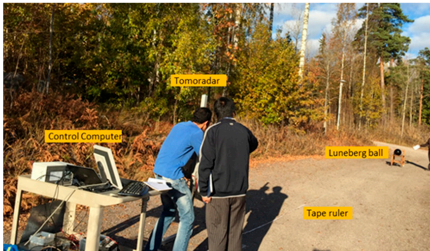
Figure 3. Range calibration.
