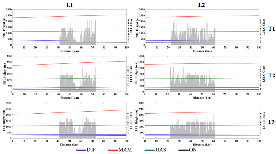
Figure S4. Same as Figure S1, but for PBL height (m).
