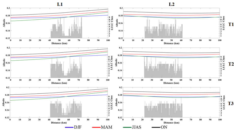
3 Figure S1. Spatial profile of albedo calculated from ERA-Interim dataset (0.125° spatial 4 resolution), varying with LULC classes for NE-SW (L1) and NW-SE (L2) transect for various 5 seasons during time periods- 1991-1999 (T1), 2000-2008 (T2), and 2009-2016 (T3). Representation of 6 LULC classes is as follows: 1- Dense Forest, 2- Open Forest, 3- Scrubs/Degraded Forest, 4- 7 Plantations, 5- Cultivable Area, 6- Built-up Area, 7- Road Rail Network, 8- River/ Waterbody, and 9- 8 Wasteland.
