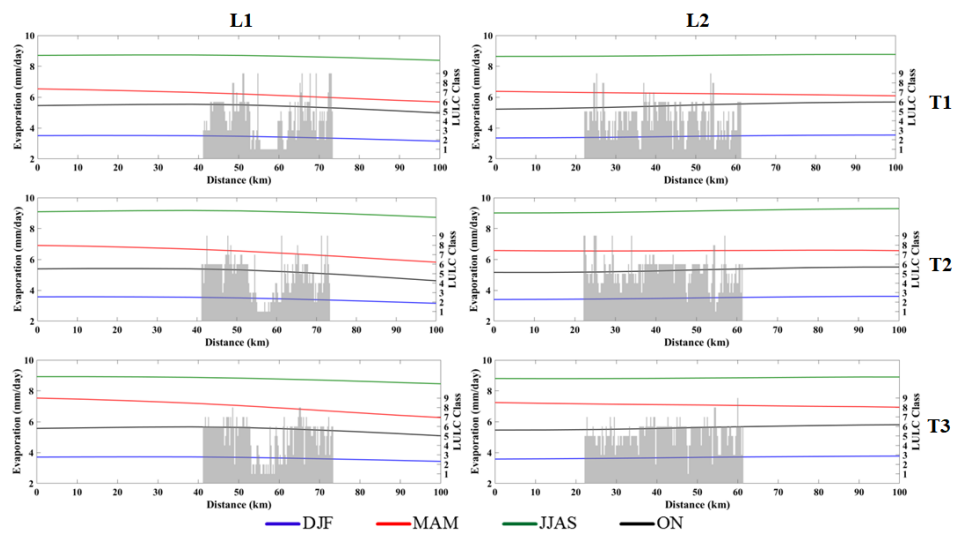
10 Figure S2. Same as Figure S1, but for evaporation (mm/day).
