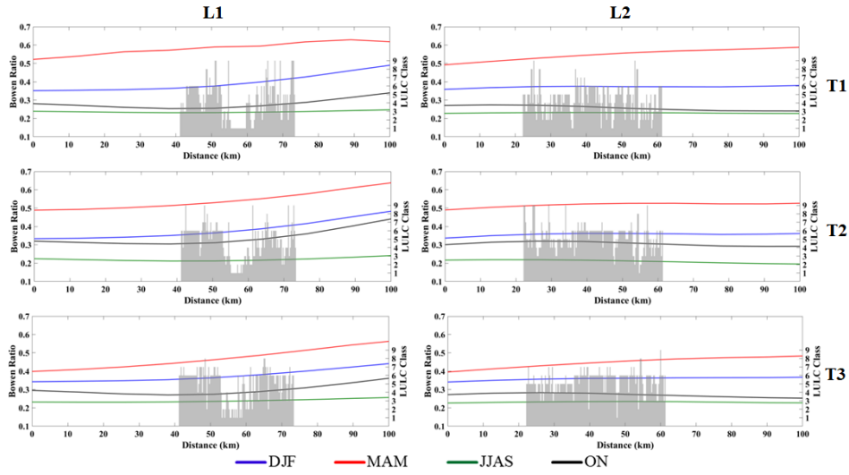
Figure S3. Same as Figure S1, but for Bowen ratio.
