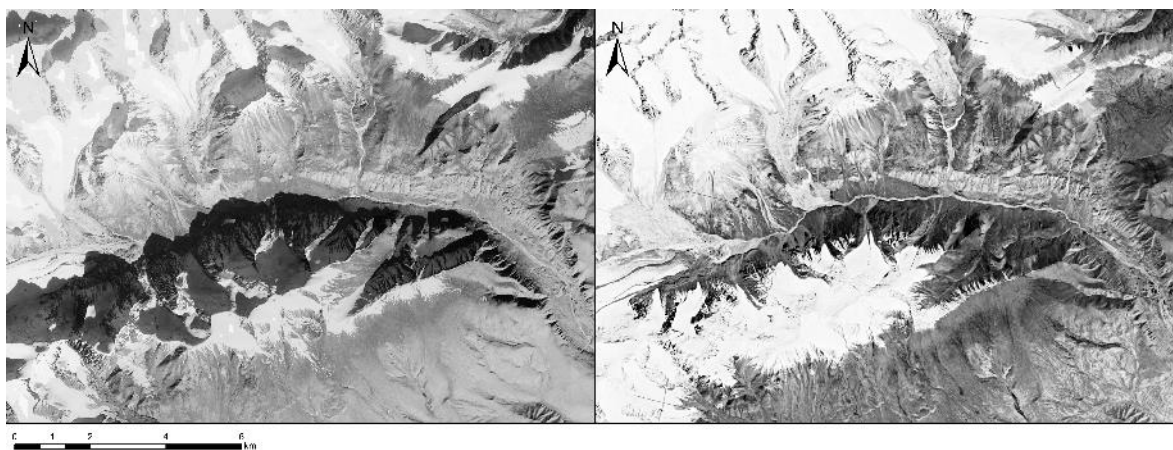
Figure S2. Snow cover comparison of the Kaindy valley in the south east of Ak-Shirak. Left image: Corona; Right image: Hexagon 1980.
