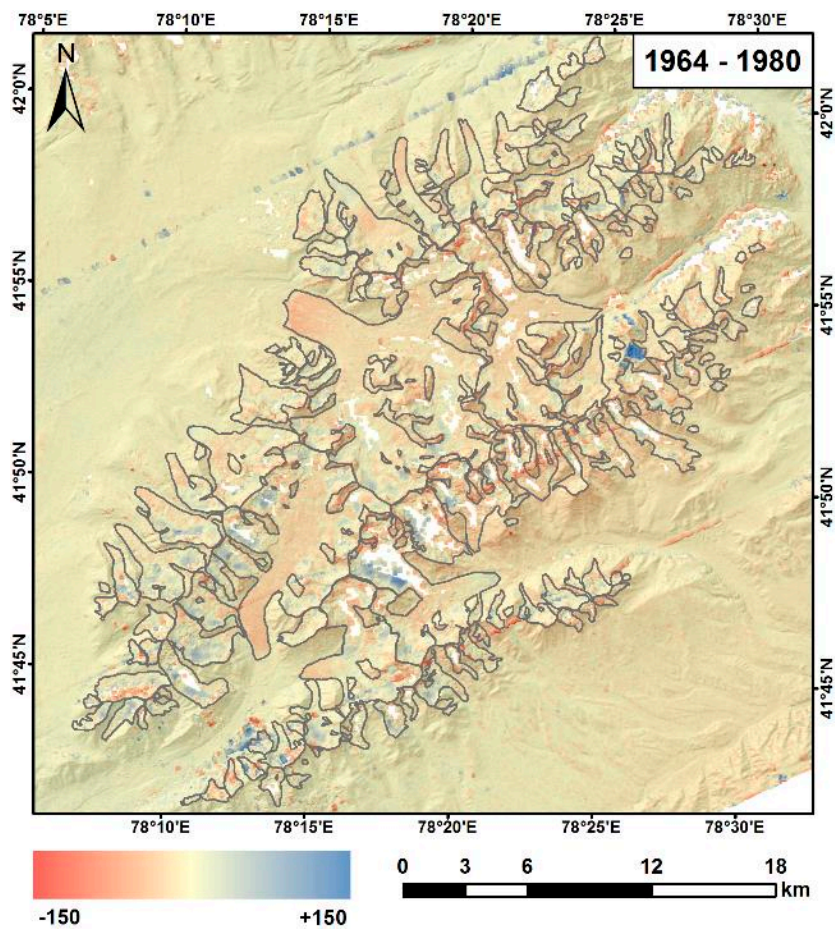
Figure S1. Elevation difference map for stable terrain and glaciers of the Ak-Shirak massif.
