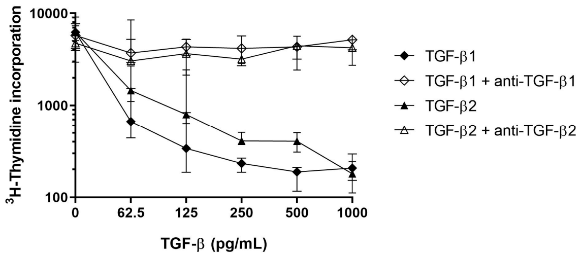
Figure S1. Effect of TGF-β1 and TGF-β2 on the inhibition of 3 H-thymidine incorporation in Mv 1 Lu cell cultures. Mv 1 Lu cells were exposed to serial dilutions of recombinant TGF-β1 or TGF-β2 with or without anti-TGF-β1 or anti-TGF-β2, respectively. Values are expressed as the median ± interquartile range. Results are representative of one experiment out of three performed with four replicates.
